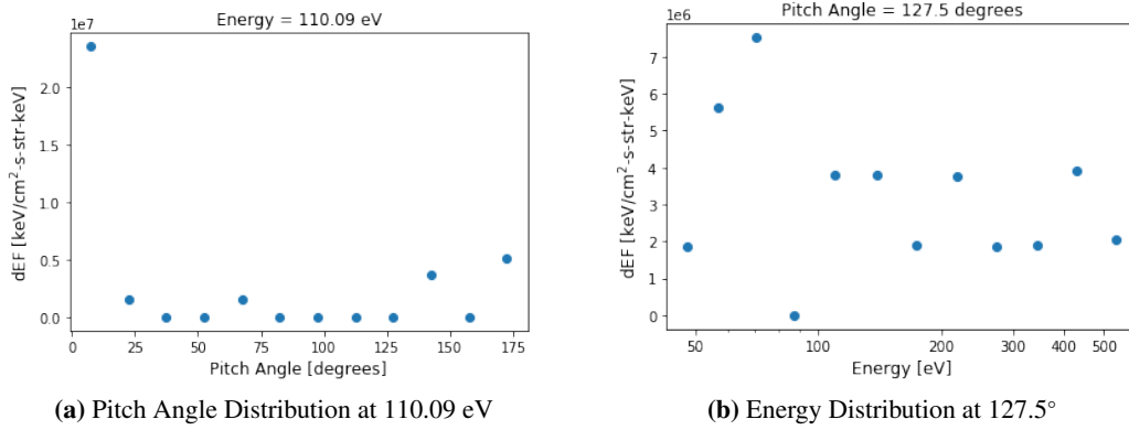
Fig. 3: a) Pitch angle distribution at an energy of 110.09 eV and, b) energy distribution at a pitch angle of 127.5^\circ as projected from the vertical and horizontal white lines in Figure 2.
