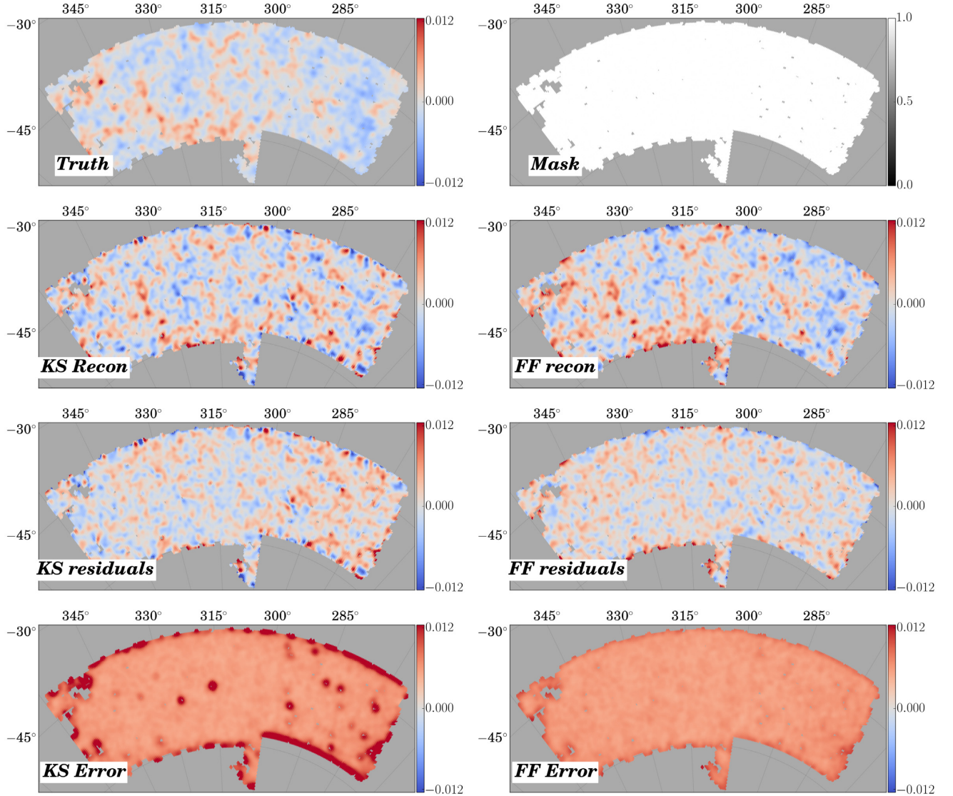
Figure 5. Reconstructions of the convergence field for the Buzzard simulation for both the direct inversion (left-hand column) and the fitting method (right-hand column). Smaller errors are present in the edge pixels of the fitted map. The fitting method also has a much more uniform residual map inside the footprint, whereas the direct inversion has a large portion of the survey with slightly larger residuals.
