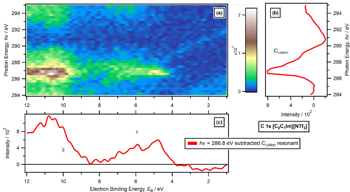
Figure 7. RAES C 1s edge data for [C 8 C 1 Im][NTf 2 ]. (a) Heat map of h\nu against E_B for the C 1s edge (produced by combining individual electron spectra taken at varying h\nu ). (b) Partial electron yield NEXAFS spectrum for the C 1s edge. (c) Subtracted C_{\text{cation}} resonant Auger electron spectrum ( h\nu = 286.8 eV). The RAES trace was produced by subtraction of non-resonant XP contributions using the procedure outlined in ESI Section 10.3. Component labels 1 and 2 are given in (c). All electron spectra were charge referenced using procedures outlined in ESI Section 5.
