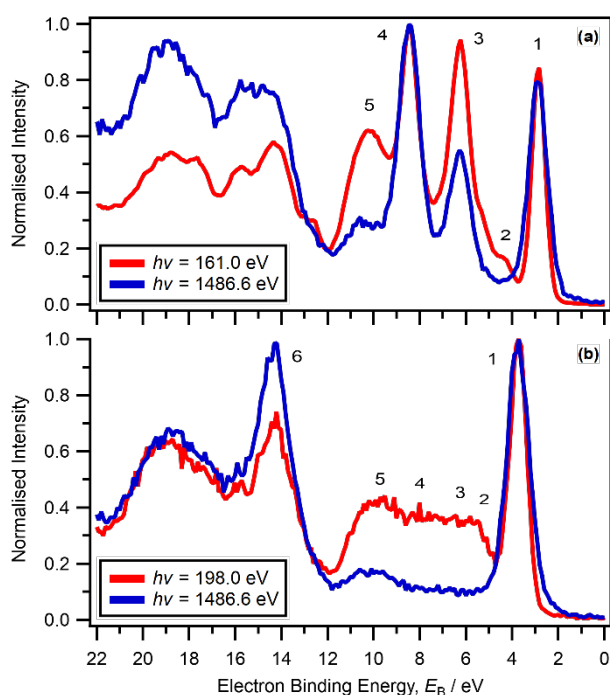
Figure 2. Variable h\nu valence XP spectra for: (a) [\text{C}_4\text{C}_1\text{Im}][\text{SCN}] at h\nu = 1486.6 eV and h\nu = 161.0 eV and (b) [\text{C}_8\text{C}_1\text{Im}]\text{Cl} at h\nu = 1486.6 eV and h\nu = 198.0 eV. All valence XP spectra were charge referenced as given in Table S3. The areas of all valence XP spectra in both graphs are normalised to the area of the most intense component in the region 0 eV < E_B < 12 eV. The numbers on each graph represent component labels.
