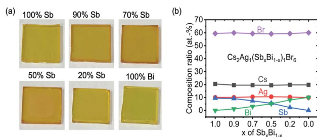
Fig. 1 (a) Photographs of the Cs 2 Ag(Sb x Bi 1-x )Br 6 films on glass under ambient lighting, with a thickness of approximately 200 nm. The Sb percentage labelled is that in the precursor solution. (b) Measurement of the bulk composition of Cs 2 Ag(Sb x Bi 1-x )Br 6 films with Rutherford Backscattering Spectrometry (fitting in Fig. S1, ESI†).
