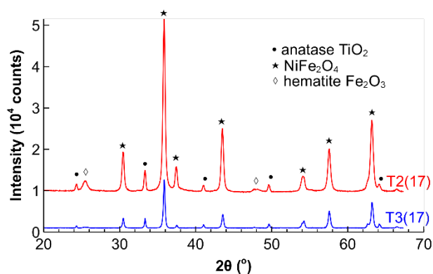
Fig. 6. Powder XRD patterns of the (a) T2(17) and (b) T3(17) catalysts.
