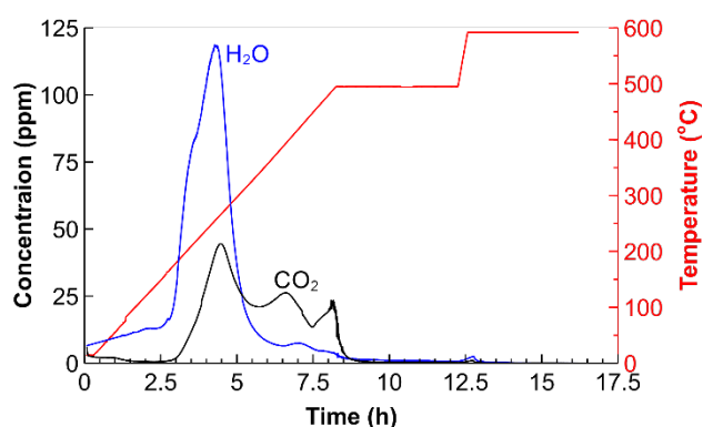
Fig. 4. CO 2 and H 2 O concentration profiles (left y-axis) and temperature profile (right y-axis) in a TPO experiment over the T3A catalyst.
