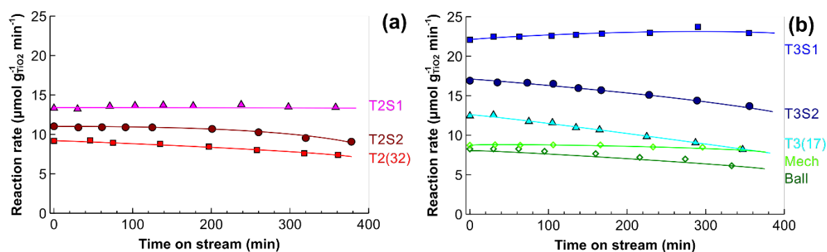
Fig. 15. Specific reaction rate as a function of time on stream over (a) core-shell and (b) core double shell catalysts as well as mechanical and ball-milled mixtures of the catalyst components. Reaction conditions: flow rate of 40 \mu\text{L min}^{-1} (50 mM 4-phenylbutyric acid, 50 mM aniline), 320 mg of the catalyst, 150^\circ\text{C} , 7 bar(g) in the RF-heated reactor.
