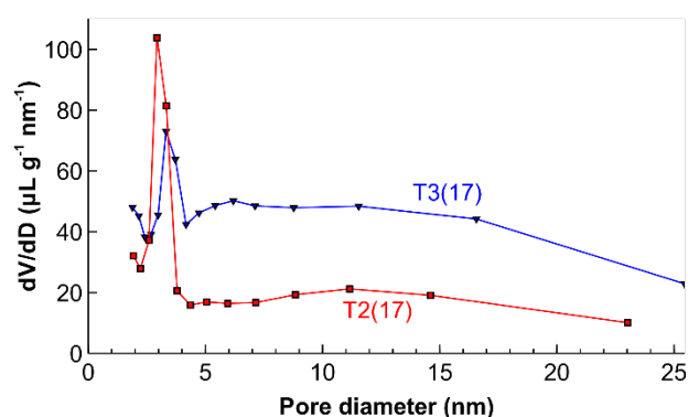
Fig. 8. Pore size distribution for the catalysts studied.
