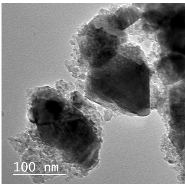
Fig. 5. TEM image of the T3(17) catalyst.
