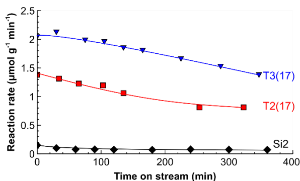
Fig. 10. Direct amide synthesis reaction rates as a function of time on stream over the magnetic composite catalysts at the flow rate of 40 μL min -1 (50 mM 4-phenylbutyric acid, 50 mM aniline), 320 mg of the catalyst, 150 °C, 7 bar(g) in the RF-heated reactor.
