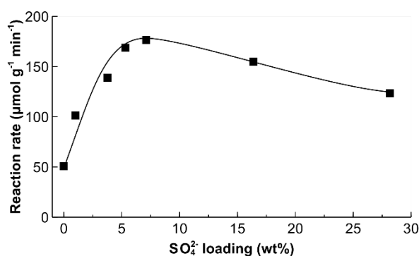
Fig. 14. Reaction rate between 4-phenylbutyric acid and aniline as a function of the SO 4 2- loading in a stirred tank reactor. Reaction conditions: 100 mL p-xylene solution of 4-phenylbutyric acid (50 mM) and aniline (50 mM), 320 mg sulfated catalyst, 6 bar(g), 200 °C.
