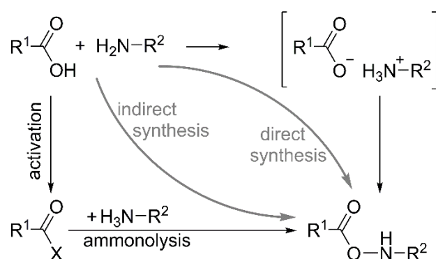
Fig. 1. General scheme of amide synthesis, adopted from refs [24,27].
