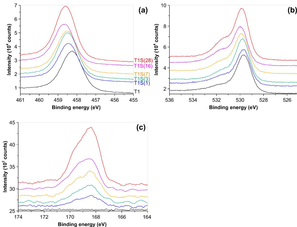
Fig. 11. X-ray photoelectron spectra of the T1S catalysts with various sulfate loading in brackets, (a)Ti 2p 3/2 , (b) O1s, (c) S 2p.
