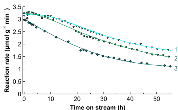
Fig. 16. Reaction rate as a function of time on stream catalysed by the T3S1 catalyst over 2 regeneration cycles with H 2 O 2 . Reaction conditions: flow rate of 40 µL min -1 (50 mM 4-phenylbutyric acid, 50 mM aniline), 320 mg of the catalyst, 150 °C, 7 bar(g) in the RF-heated reactor.
