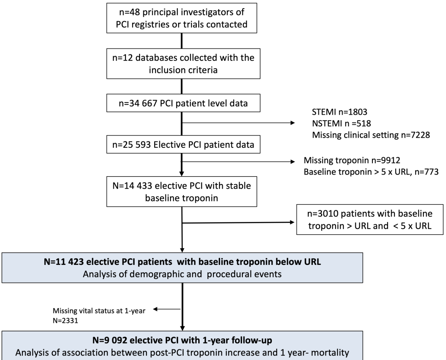
Figure 1: Consort diagram
