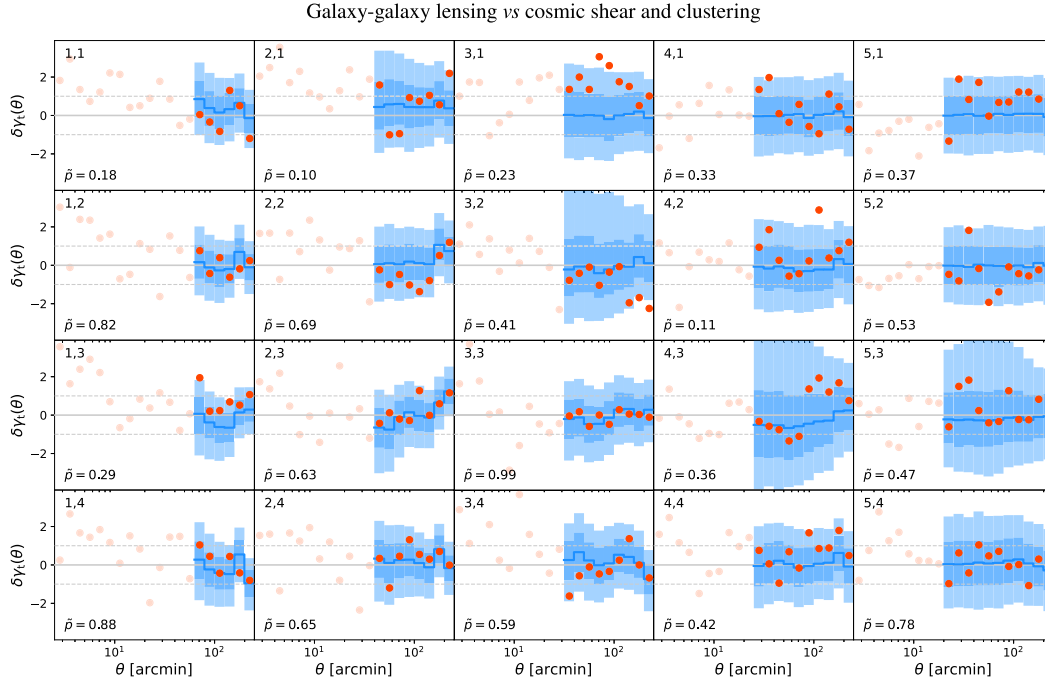
Figure B1. PPD for galaxy–galaxy lensing, conditioned on the posterior from cosmic shear and clustering. See Fig. 2 for explanation of bands.
