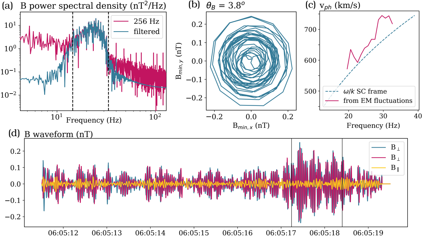
Fig. 6. Data analysis of the SWF data product from 24 June 2020, 06:05:15.5. (a) Power spectral density of the 256 Hz magnetic-field in pink and the band-pass filtered spectral density in blue; (b) A hodogram of the selected wave packet with the highest amplitude, representing the interval marked with black lines in the waveform data shown in (d); (c) Phase velocity determined from the electric and magnetic field fluctuations (Kretzschmar et al. 2021) compared to the theoretical prediction ( \omega/k ) calculated from the wave frequency in the SC and solar-wind reference frame. We assume the solar wind with a radial velocity of 350 km/s; (d) The snapshot waveform interval (SWF), where the \mathbf{B} components are given in the background magnetic-field-aligned frame. The yellow colour denotes the parallel component.
