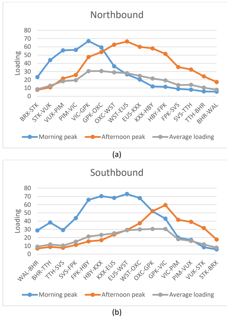
Figure 3-3: Variation of mean passenger load for morning peak, afternoon peak and day average at different stations: (a) northbound trains and (b) southbound trains.
