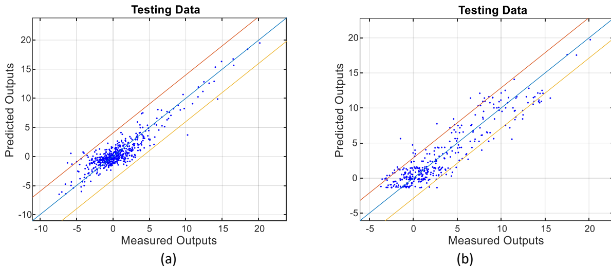
Figure 5-5: Measured versus predicted outputs using developed local models (with \pm 10\% error bands): (a) the weather local model and (b) the event local model.
