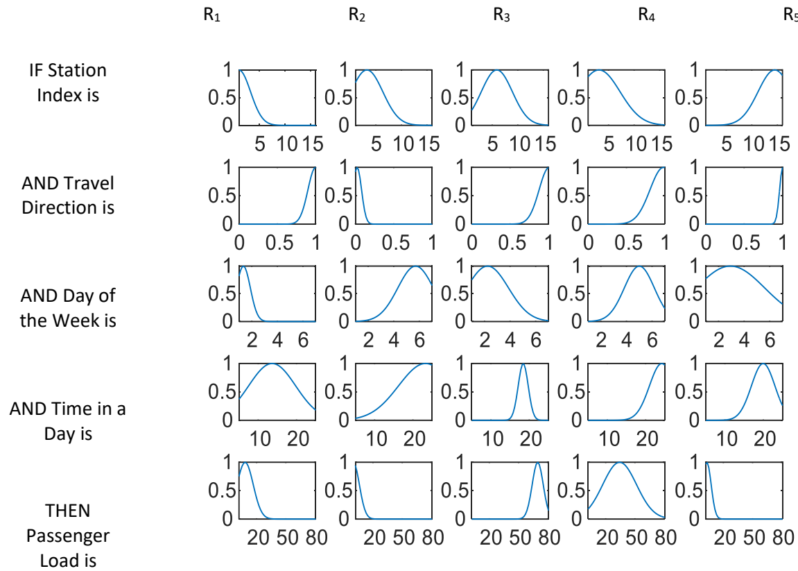
Figure 5-4. Examples of fuzzy rules of the global passenger flow model.
