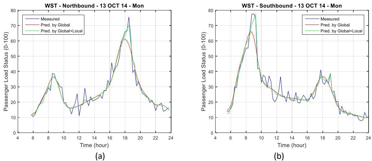
Figure 5-6: Prediction of passenger load on trains in a rainy day, 13 th October 2014, Monday: (a) northbound trains approaching Warren Street and (b) southbound trains leaving Warren Street.
