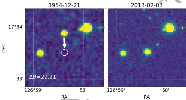
Figure 7. POSS-1 (left) and PanSTARRS-1 (right) sky survey images taken 59 years apart, long enough for EPIC 211817229 to have moved about d\theta \approx 22'' along the direction of the white arrow. The white circle shows a clear view along the line of sight to the position of the target in the right image, helpful to rule out a background eclipsing binary scenario.
