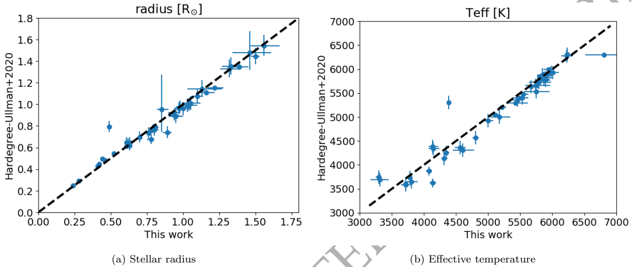
Figure 4. Comparison of stellar radius and T_{\text{eff}} derived from this work and reported in Hardegree-Ullman et al. (2020). The black dashed lines represent one-to-one correspondence ( x=y ). Our results are consistent with those of Hardegree-Ullman et al. (2020) at the 1- \sigma level.
