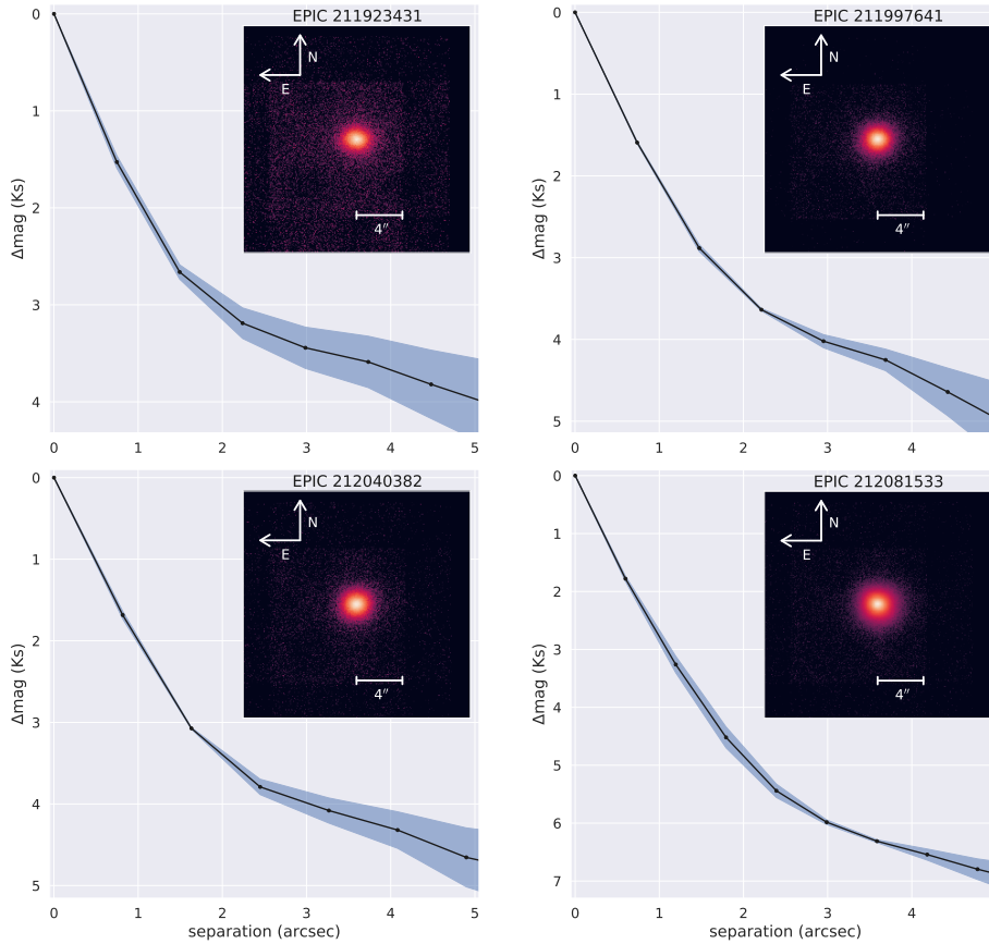
Figure 2. Adaptive optics images of EPIC 211923431, EPIC 211997641, EPIC 212040382, and EPIC 212081533 taken with the ShARC5 camera on the Shane 3-meter telescope at Lick Observatory. For each image, we also present a contrast curve generated by calculating the median values (solid lines) and root-mean-square errors (blue, shaded regions) in annuli centered on each target, where the bin width of each annulus is equal to the full width at half max of the point spread function.
