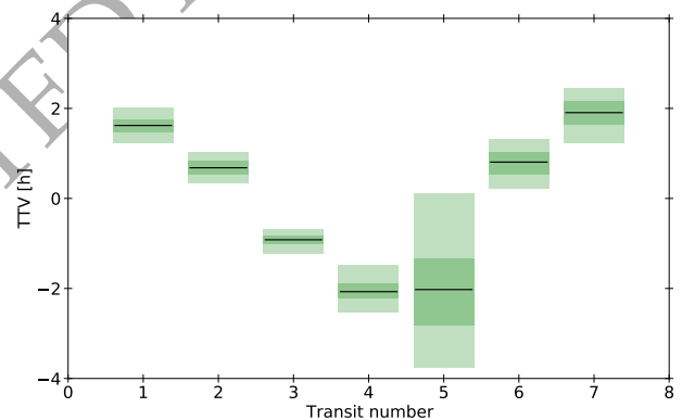
Figure 11. Transit timing variations in EPIC 212058012 where only one transiting planet is hitherto known. The black lines mark the median values and the 68% and 99% central posterior percentiles are indicated by the dark and light shaded area, respectively.
