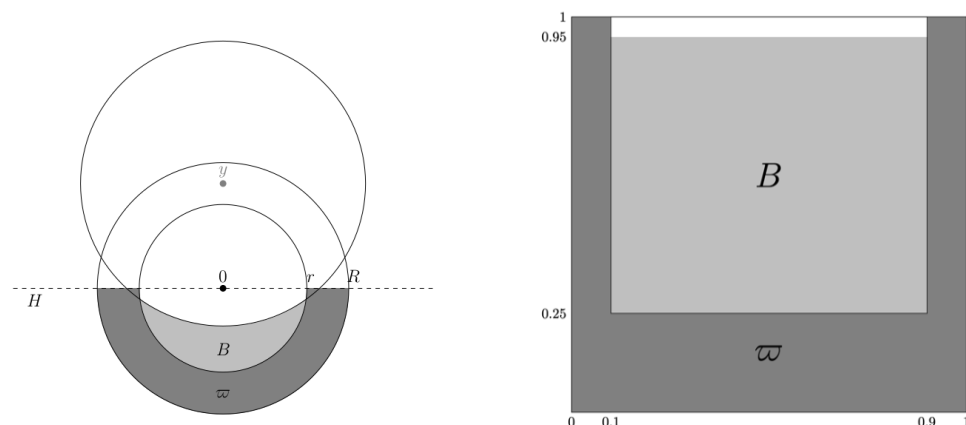
FIG. 3.1. Configurations from [10] satisfying the convexity condition necessary for Lemma 3.2. Left panel: specific configuration defined in (3.3). Right panel: configuration also satisfying the bound (3.4).
