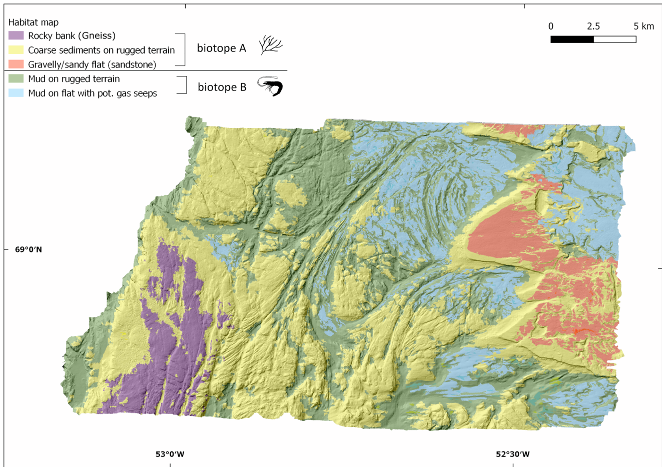
Figure 11. Benthic habitat map superimposed on a hillshade terrain model, showing distribution of identified habitats and associated biotopes in Disko Bay study area. CRS: WGS 84.
