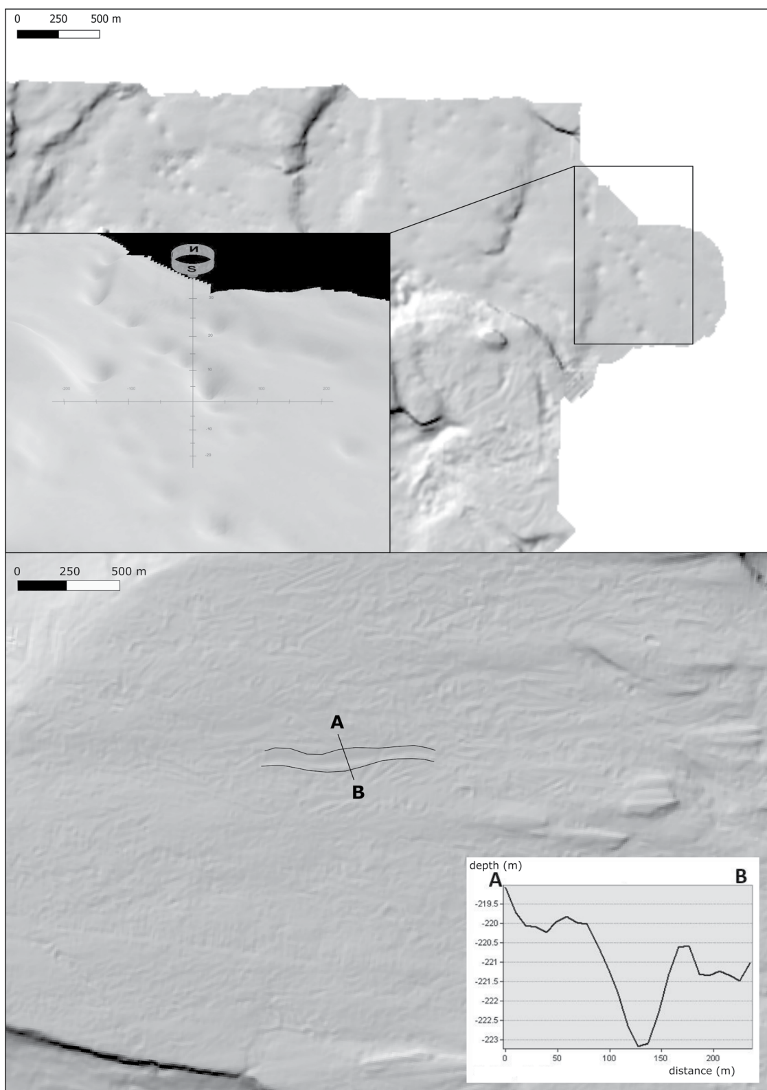
Figure 7. Examples of pockmarks (top) and iceberg ploughmarks (bottom) in the eastern part of the study area (hillshade terrain model). Insert image on top shows 3D terrain model of the NE corner of the study area.
