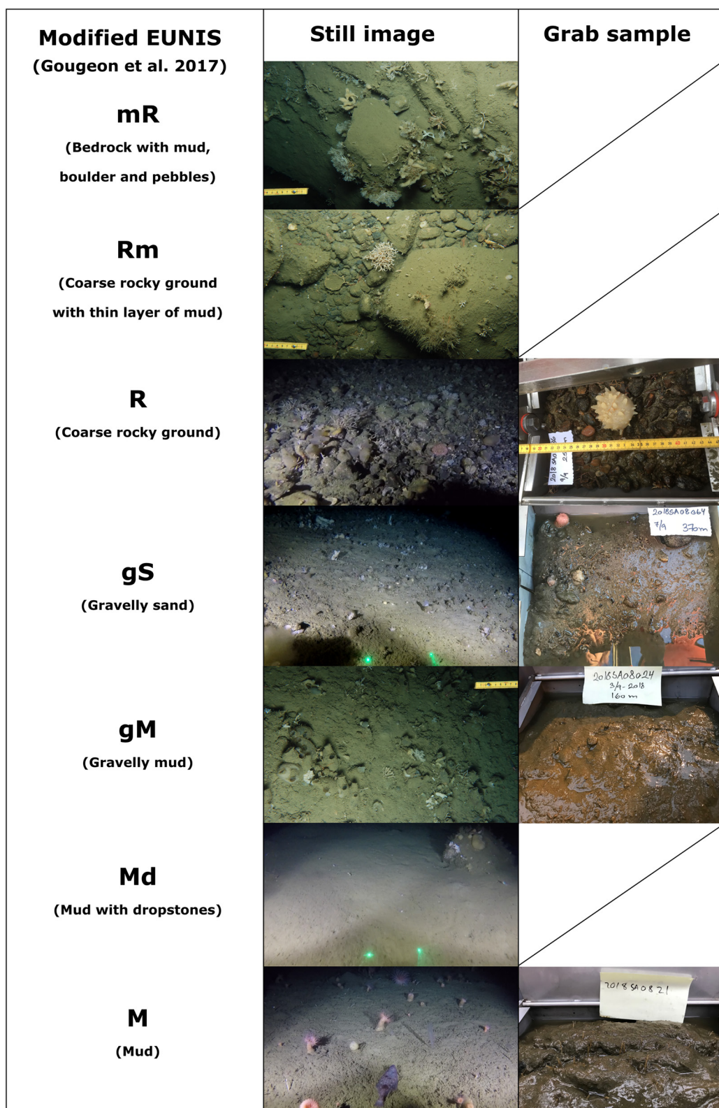
Figure 5. Images illustrating each of the seven sediment categories identified in Disko Bay pilot area, consisting of still images from drop camera/video sled and pictures of grab samples. Sediment categories follow the scheme of Gougeon et al. (2017).
