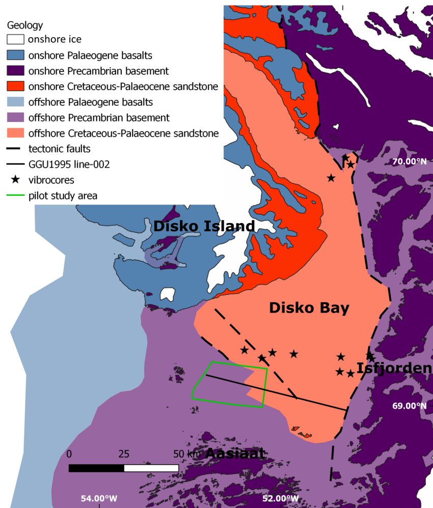
Figure 1. Pre-Quaternary geological setting of the Disko Bay region (modified from Nielsen et al., 2014). Full tones represent onshore geology and half tones represent offshore geology. Dashed black lines indicate tectonic faults. Solid black line indicates position of the seismic profile GGU1995 line-002 and solid black stars indicate locations of vibrocores from RRS James Clark Ross cruise (JR175; in Streuff et al., 2017). Green box marks the outline of the pilot study area. Coordinate Reference System (CRS): WGS 84.
