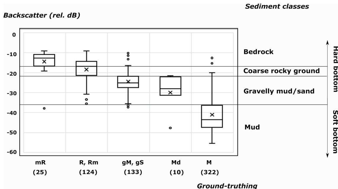
Figure 8. Box plot showing sediment classes identified from ground-truthing in relation to backscatter intensity (dB). Horizontal lines in boxes indicate median values and crosses are at mean values; boxes indicate quartiles, whiskers indicate standard deviation and black circles are outliers. Sample numbers for each category are shown in the brackets (bottom). Ground-truth labels: mR—bedrock with mud, boulder and pebbles, R—coarse rocky ground, Rm—coarse rocky ground with thin layer of mud, gS—gravelly sand, gM—gravelly mud, Md—mud with dropstones, M—mud.
