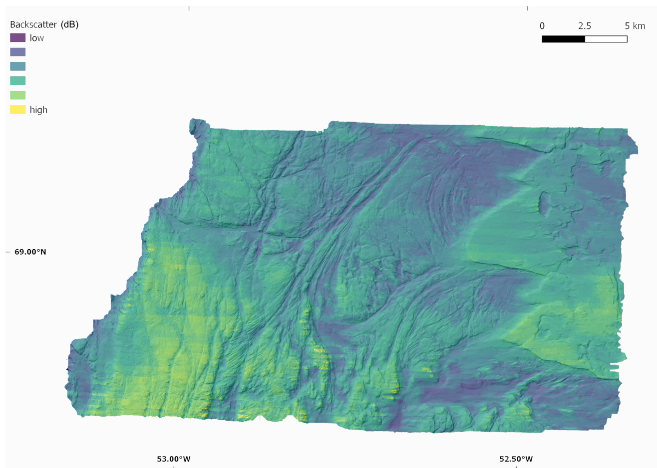
Figure 4. Backscatter mosaic (dB) of 10 \times 10 m resolution superimposed on a hillshade terrain model in Disko Bay study area. Maximum backscatter intensity is -9 dB and minimum backscatter intensity is -56 dB. CRS: WGS 84.
