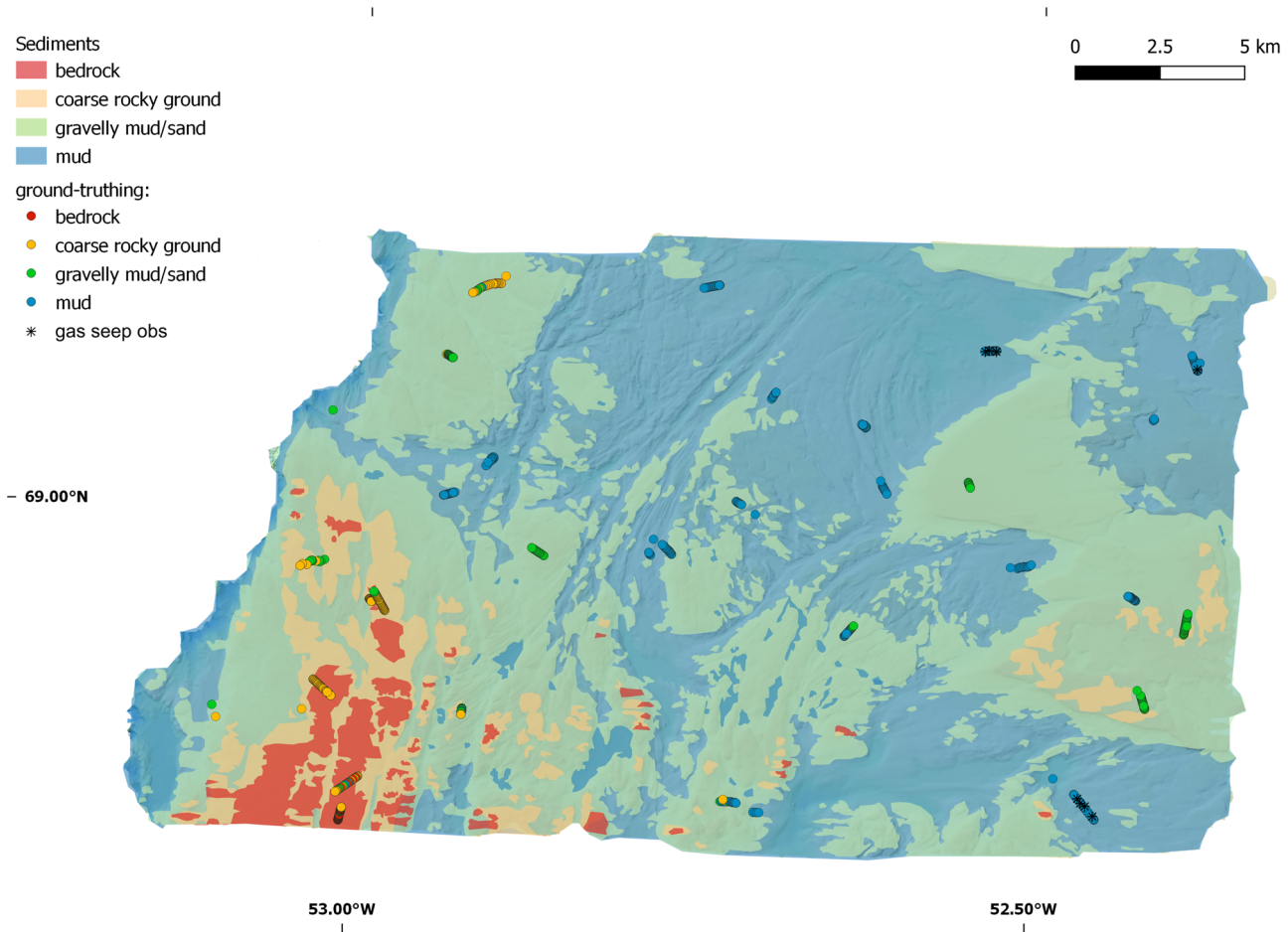
Figure 9. Backscatter-derived sediment map superimposed on a hillshade terrain model, showing distribution of identified sediment types in Disko Bay study area together with ground-truth stations and gas seep observations (see legend). CRS: WGS 84.
