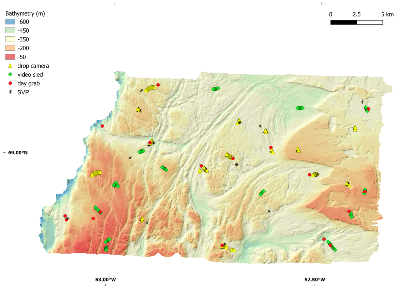
Figure 3. Bathymetric grid (m) of 10 \times 10 m resolution superimposed on a hillshade terrain model with locations of ground-truth stations/transects including Sound Velocity Profiles (SVP) in Disko Bay study area (see legend). CRS: WGS 84.
