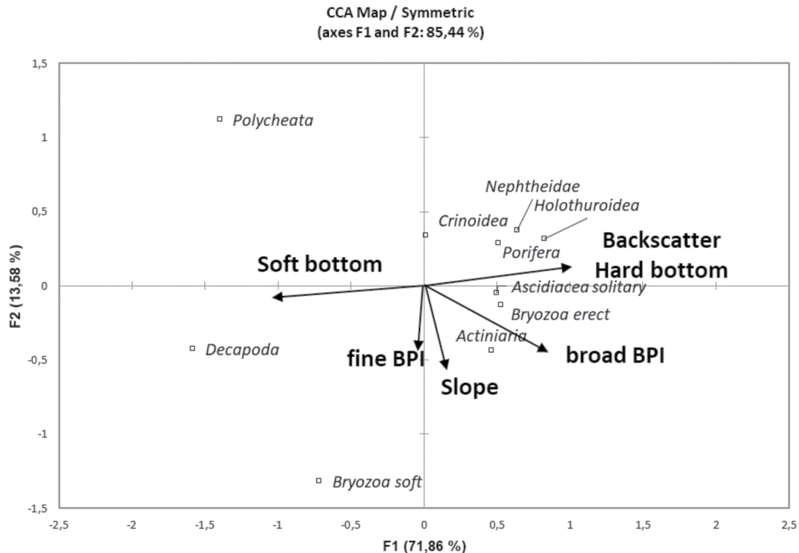
Figure 10. Ordination diagram of benthic taxa and independent environmental variables along two CCA axes. Groups plotting to the right are associated with hard bottom (i.e., biotope A) and groups plotting to the left are associated with soft bottom (i.e., biotope B).
