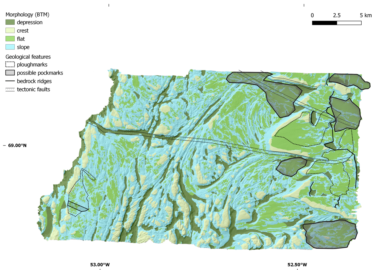
Figure 6. Morphology map showing distinct terrain features using broad BTM classification together with geological features identified in Disko Bay study area (Krawczyk, Jensen, et al., 2019). CRS: WGS 84.
