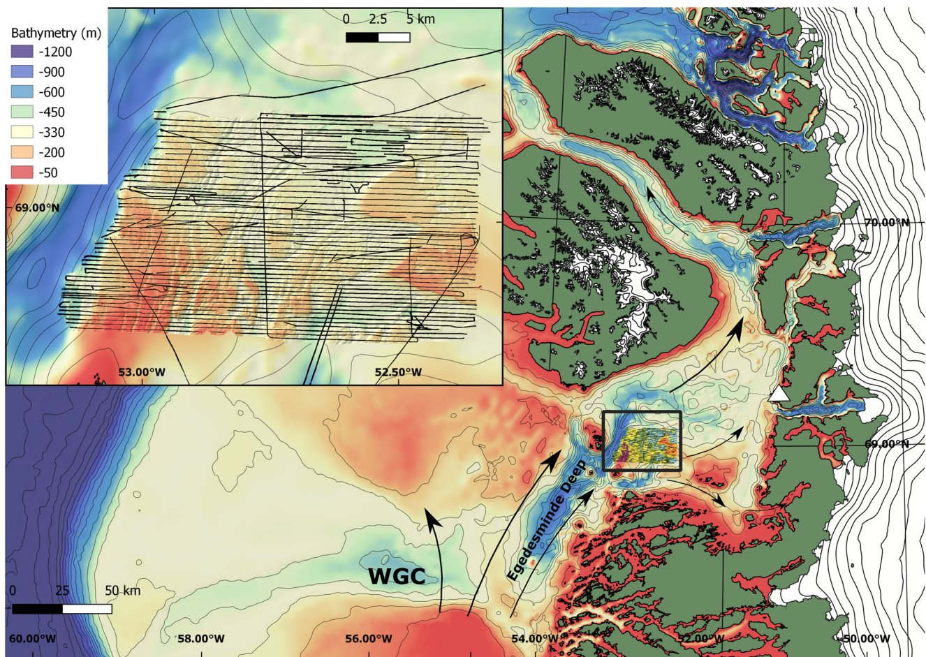
Figure 2. Bathymetry (m) of central West Greenland shelf, that is, Disko Bay region superimposed on a relief map. Source: BedMachine v3 (Morlighem et al., 2017). The arrows indicate the approximate flow of the West Greenland Current (adapted from Andersen, 1981). The white triangle shows Ilulissat harbor. White color on land indicates ice. Insert map shows the tracklines of this pilot study survey overlaying the survey bathymetric grid (see Figure 3). CRS: WGS 84.
