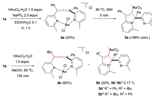
Scheme 3 Synthesis of Au(III)-complexes 4a–b and 5a–b.
