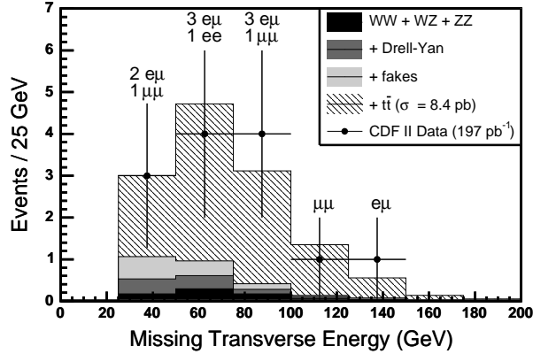
FIG. 2: \cancel{E}_T for events from the DIL analysis with H_T > 200 GeV and \geq 2 jets.
