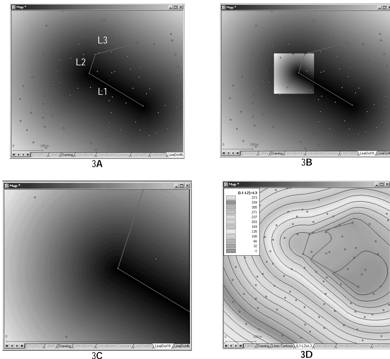
Figure 3: (3A) A polyline, made of segments L1, L2 and L3, is used to demonstrate the capabilities of Map Calculus-enabled GIS. In this image, the distance function is calculated at a scale of about 1:4000. Once the user zooms in to a smaller area (3B), the system calculates the new values of the surface for that specific area, and, as the next image (3C) demonstrates there is no “pixelation” of the surface (note the scale bar). In 3D, the following composite function was calculated: (\text{Dist L1} - \text{Dist L2}) + \text{Dist L3} . The resulting surface was calculated directly from the final function and not by creating intermediate surfaces.
