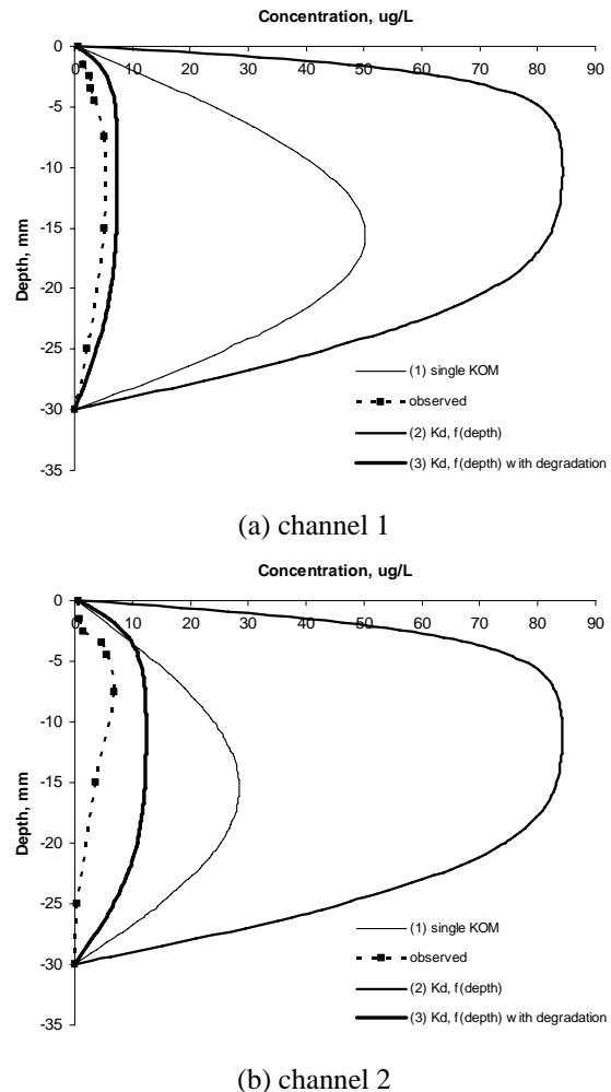
Figure 2: Concentration-depth profiles for lindane under dark conditions for both channels. Data from (Allan et al. 2004)
