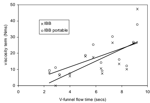
Figure 22: Relationships between plastic viscosity/viscosity term and V-funnel flow time for concrete mixtures
