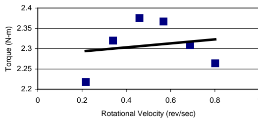
Mixture BTRD1M2-Mortar (Close-up)
