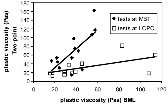
(b) BML/Two-point
