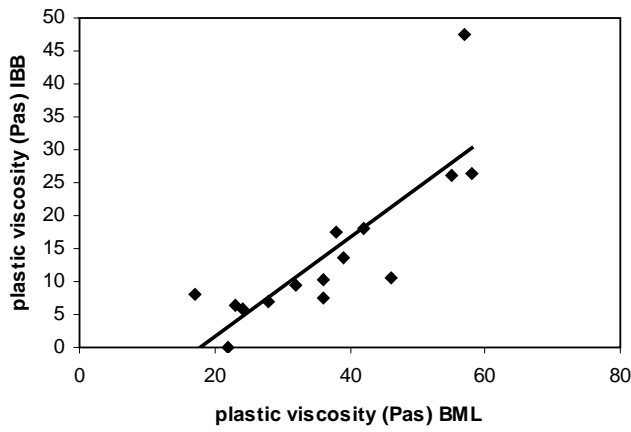
(c) plastic viscosity - IBB vs BML
