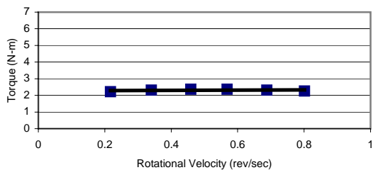
Mixture BTRD1M2-Mortar
