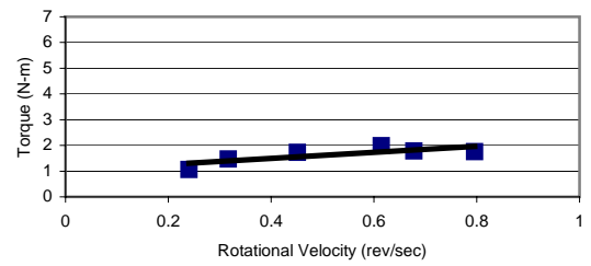
Mixture BTRD3M2-Concrete
