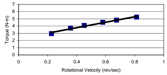
Mixture BTRD3M1-Concrete
