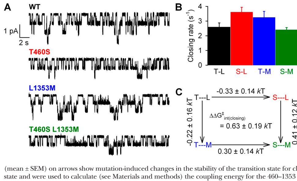
Figure 2. Effect of mutations at positions 460 and 1353 on channel closing rates. (A) Representative traces of multichannel recordings of prephosphorylated WT and mutant CFTR channels, used to determine burst duration. Downward deflection indicates inward current. (B) Closing rates of WT and mutant CFTR channels, defined as the inverse of the mean burst duration (see Materials and methods). (C) Thermodynamic mutant cycle for target pair T460-L1353 built on the closing rates from B; each corner is represented by the side chains at positions 460 and 1353, respectively. \Delta\Delta G^0 values (mean \pm SEM) on arrows show mutation-induced changes in the stability of the transition state for closure with respect to the open ground state and were used to calculate (see Materials and methods) the coupling energy for the 460–1353 interaction ( \Delta\Delta G_{\text{int(closing)}}^{\ddagger} ).
