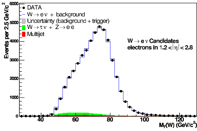
FIG. 2 (color online). M_T distribution for W \rightarrow e\nu candidates (●). The histogram is the sum of the expected background and the predicted (from simulation) signal spectrum.
