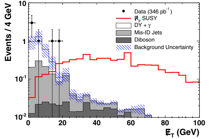
FIG. 2 (color online). \cancel{E}_T for events in the trilepton signal samples. For comparison, an R_p SUSY sample is shown with M(\tilde{\chi}_1^0) = 99 \text{ GeV}/c^2 .
