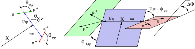
FIG. 2 (color online). Definition of the decay angles. The polar angles ( \theta ) are calculated from the parent momenta and the child momenta in the corresponding parent rest frame.
