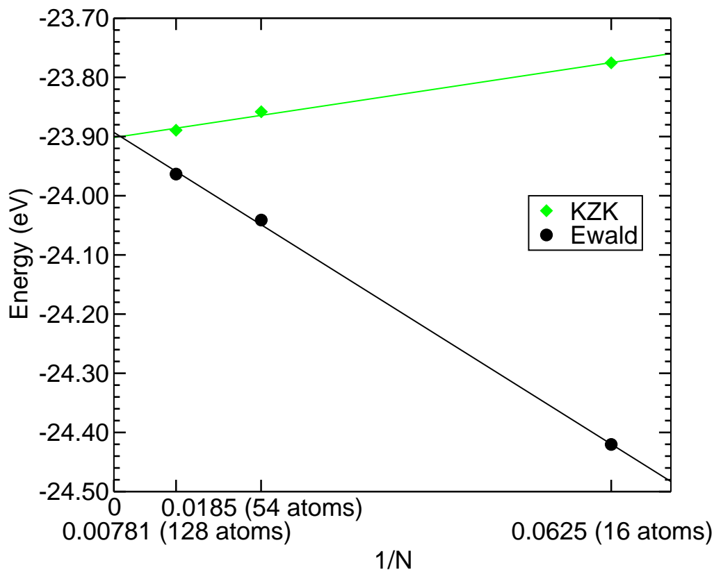
Figure 4.5: Energy vs. Supercell size: LiH Bulk. Shown are the original DMC total energies computed using the Ewald method and the values including the KZK correction. Both data sets have been fitted to Equation 3.35 to provide an infinite cell extrapolation. The statistical errors on each point are smaller than the symbols.
