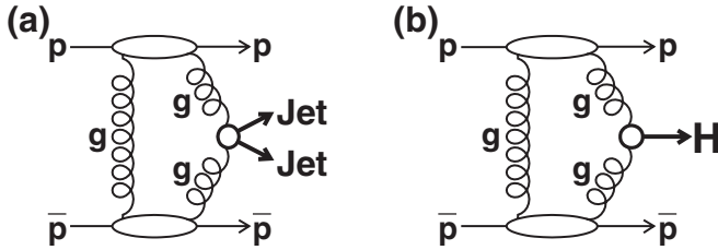
FIG. 2. Leading order diagrams for (a) exclusive dijet and (b) exclusive Higgs boson production in \bar{p}p collisions.
