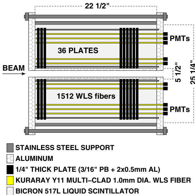
FIG. 4 (color online). Schematic cross sectional view of one of the two forward MiniPlug calorimeters installed in CDF II.
