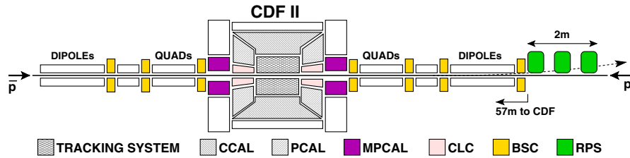
FIG. 3 (color online). Schematic drawing (not to scale) of the CDF II detector.
