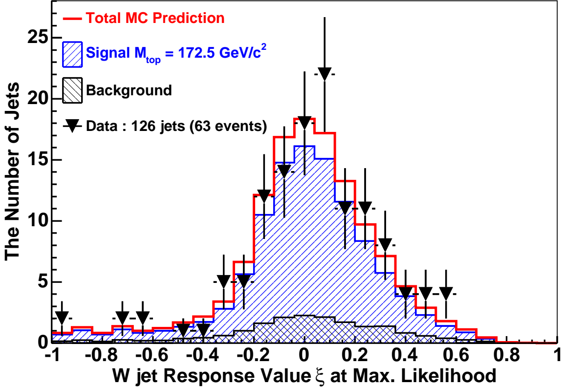
FIG. 25: Comparison of the W -jet response variable \xi between the data (triangles) and the simulation (histograms show signal, background, and total(= signal + background)). The means and resolutions are summarized in Table II.
