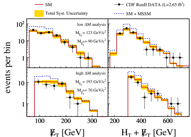
FIG. 1 (color online). Measured \cancel{E}_T and H_T + \cancel{E}_T distributions (black dots) for low- \Delta M (top) and high- \Delta M analyses (bottom), compared to the SM predictions (solid lines) and the SM + MSSM predictions (dashed lines). The shaded bands show the total systematic uncertainty on the SM predictions.
