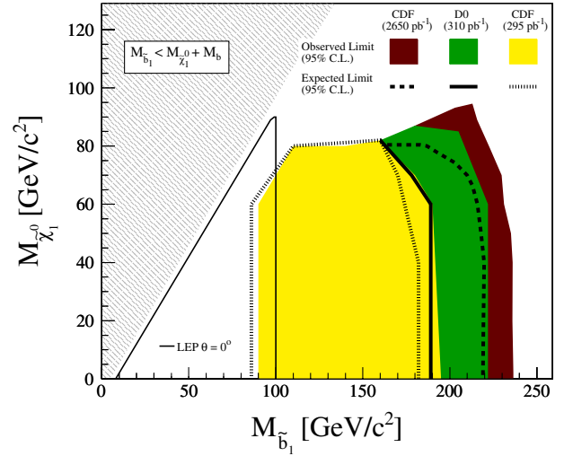
FIG. 2 (color online). Exclusion plane at 95% C.L. as a function of sbottom and neutralino masses. The observed and expected upper limits from this analysis are compared to previous results from CDF and D0 experiments at the Tevatron in Run II [4,5], and from LEP [27] experiments at CERN with squark mixing angle \theta = 0^\circ . The hatched area indicates the kinematically prohibited region in the plane.
