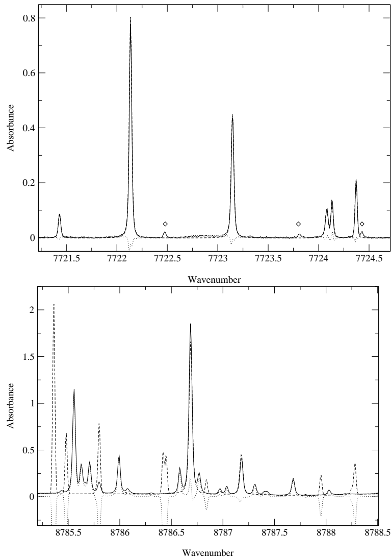
Fig. 1. Comparison of the spectrum of Schermaul et al. [9] with that predicted by HITRAN-2004 [1] for the same conditions. Solid line – experiment; long dashed line – simulation; short dashed line – residual. Diamonds on the upper plot denote lines missing in HITRAN-2004.
