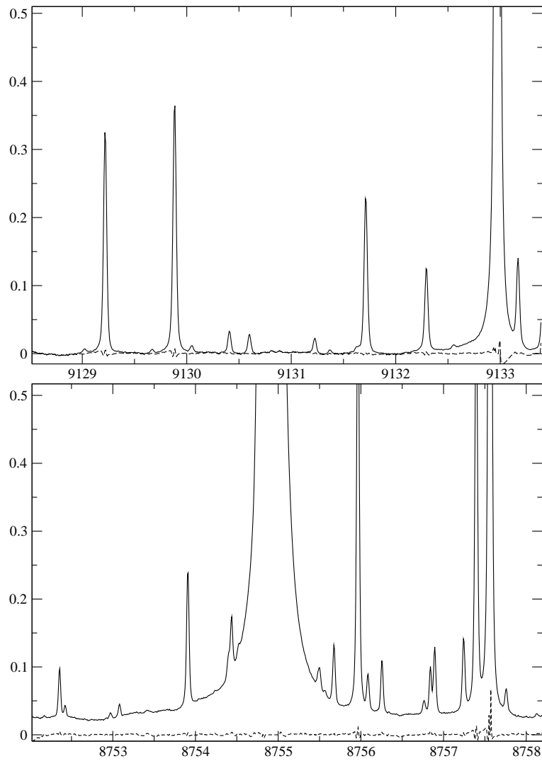
Fig. 2. Two portions of the experimental spectrum. The dashed line is the residual in our fit.
