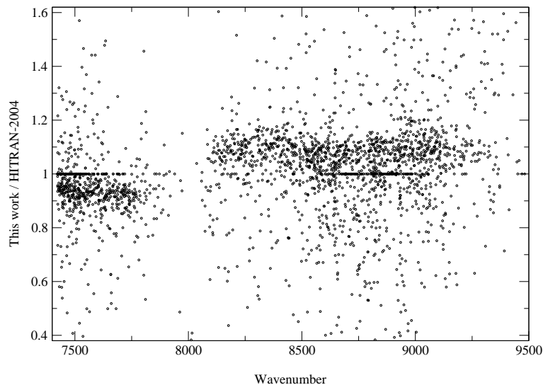
Fig. 3. Comparison of the line intensities from this work with those from the HITRAN-2004 database.
