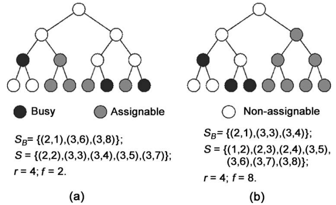
Fig. 2. Occupancy statuses of two 3-layer code trees.
