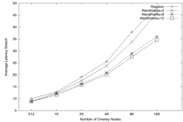
Fig. 8. Stretch for a 2-dimensional CAN; topology PLRG2; #levels=1
