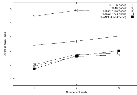
Fig. 2. Effect of number of levels (#landmarks = 12)
