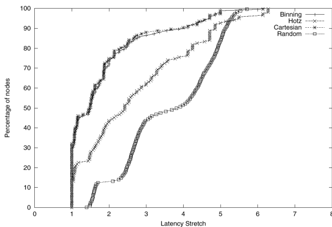
Fig. 10. Effect of Number of Landmarks and Topology
