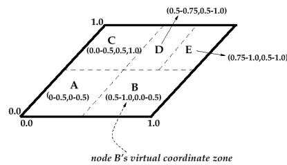
Fig. 5. Example 2-d coordinate overlay with 5 nodes
