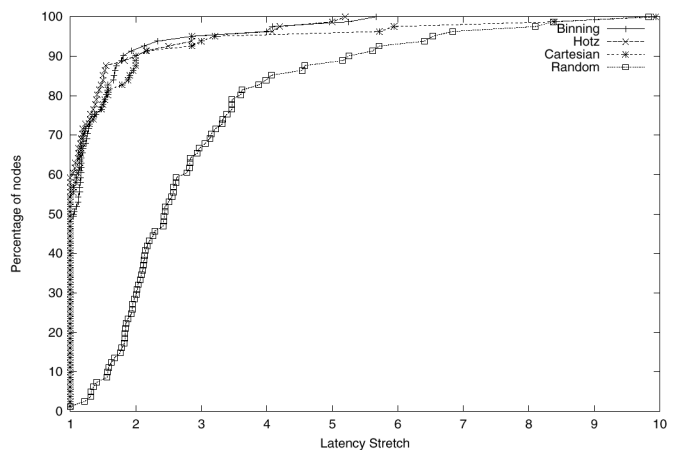
Fig. 11. Cumulative distribution of Latency Stretch
