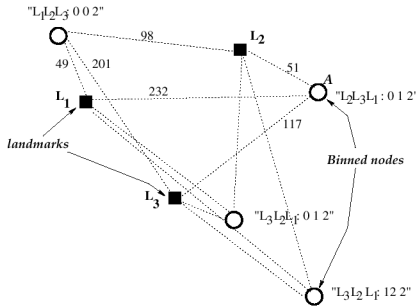
Fig. 1. Distributed binning
