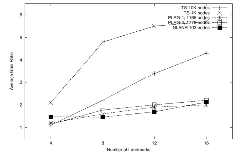
Fig. 3. Effect of number of landmarks (#levels = 1)
