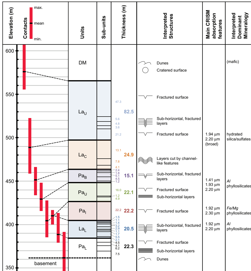
Fig. 9. Graphic sedimentary log of LTDs in the northern wall of the Coprates Catena trough. Elevation contacts (mean, minimum, and maximum) are calculated for the entire contact on the northern wall, whereas the elevation values for the units are taken from a single profile shown in Fig. 5a. Thicknesses of units and possible sub-units are measured from the single profile, whereas the structures and main CRISM absorption features are representative of the unit as a whole.
