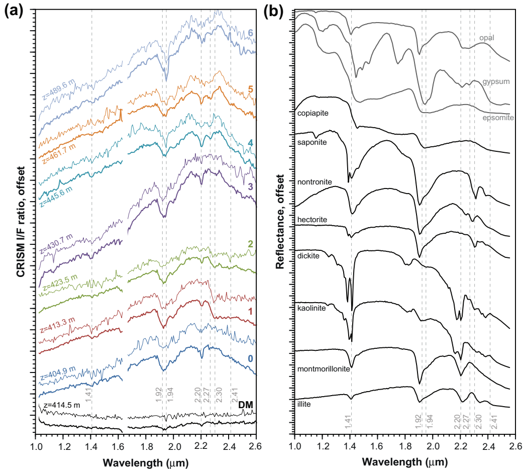
Fig. 7. CRISM spectral ratios and comparison mineral reflectance spectra. (a) CRISM ratios made using the numerator and denominators shown in Fig. 6, taken at the locations shown in Fig. 4a. Thick lines represent the RoI spectra and thin lines represent the individual spectra ( 3 \times 3 pixel average). For each ratio the elevation at the pixel average location is also given. DM is the dark mantling material discussed in the text and does not form part of the CRISM sequence study. Data are not shown at around 1.00 and 1.65 \mu\text{m} due to known instrument artifacts (e.g. Fueten et al., 2010; Lichtenberg et al., 2010). Dashed vertical lines correspond with absorption wavelengths used for identification. (b) Laboratory reflectance spectra of candidate minerals showing probable species responsible for low elevation (black lines) and higher elevation (gray lines) spectral features. All spectra are from the USGS spectral library splib06a (Clark et al., 2007), with reference spectra for illite (GDS4), montmorillonite (SWy-1), kaolinite (CM9), dickite (NMNH106242), hectorite (SHCa-1), nontronite (SWa-1.a), saponite (SapCa-1), copiapite (GDS21), epsomite (GDS149), gypsum (HS333.3B), and opal (TM8896).
