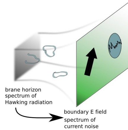
FIG. 1: Sketch of the AdS geometry with boundary current fluctuations: The AdS brane geometry is modified by the application of an in-plane electric field at the boundary. Hawking radiation from the modified horizon propagates to the boundary where it induces current fluctuations. These fluctuations satisfy an equilibrium-like fluctuation dissipation relation at a temperature T_* = [T^4 + \hbar^4 c^4 e^2 E^2 / (\pi k_B)^4]^{1/4} , interpolating between established low- and high-field limits.
