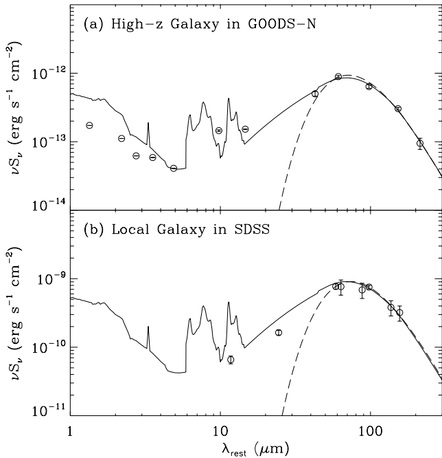
Figure 1. Example SEDs for (a) a high- z galaxy in GOODS-N with L_{\text{IR}} = 6.7 \times 10^{11} (L_{\odot}) , T_{\text{dust}} = 37 \text{ K} and z = 0.64 ; (b) a local galaxy in SDSS with L_{\text{IR}} = 4.9 \times 10^{11} (L_{\odot}) , T_{\text{dust}} = 35 \text{ K} and z = 0.02 . The best-fitting CE01 and MBB models are indicated by solid and dashed lines, respectively.
