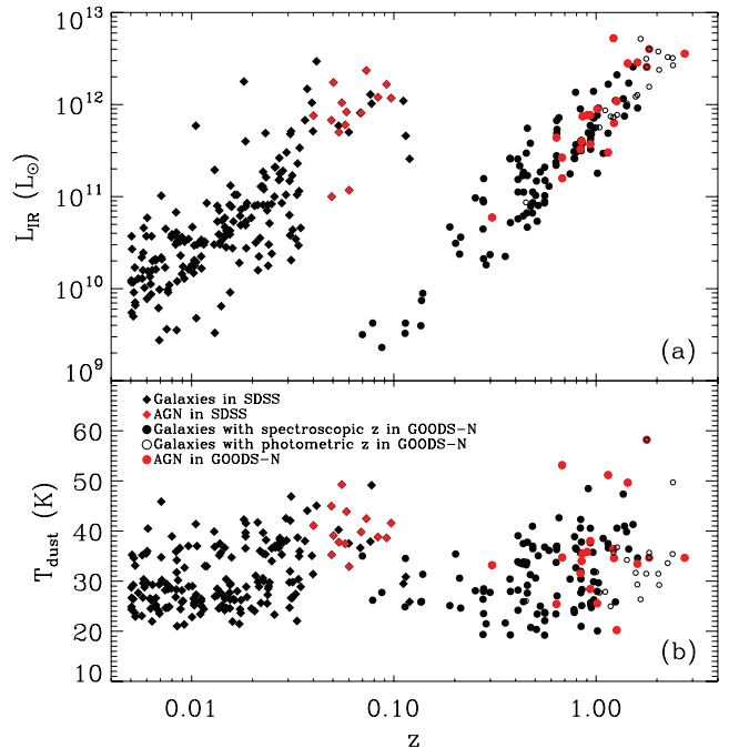
Figure 2. (a) L_{\text{IR}} and (b) T_{\text{dust}} for 140 galaxies in GOODS-N (circles) and 190 galaxies in SDSS (diamonds) versus redshift. Galaxies with spectroscopic and photometric redshifts are filled and open circles, respectively. Galaxies hosting AGN are indicated by red symbols.
