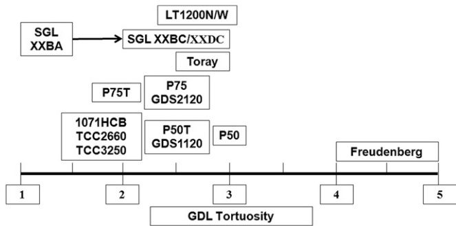
Fig. 12. Tortuosity of commercial GDLs.
