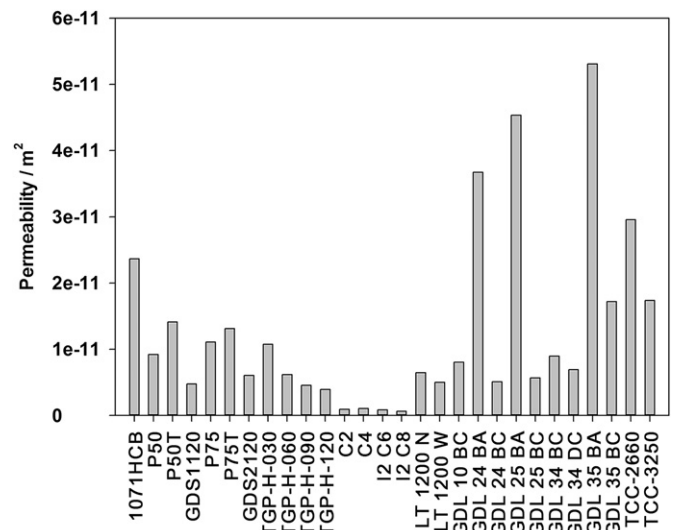
Fig. 18. GDL permeability as measured using mercury porosimeter.
