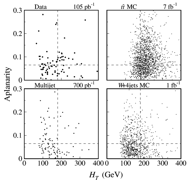
FIG. 1. Distributions of \mathcal{A} vs H_T for \ell + \text{jets} data events compared to expectations for higher luminosity samples of t\bar{t} ( m_t = 170 \text{ GeV}/c^2 ), multijet, and W + 4 jets backgrounds. The dashed lines represent the threshold values used for the selection.
