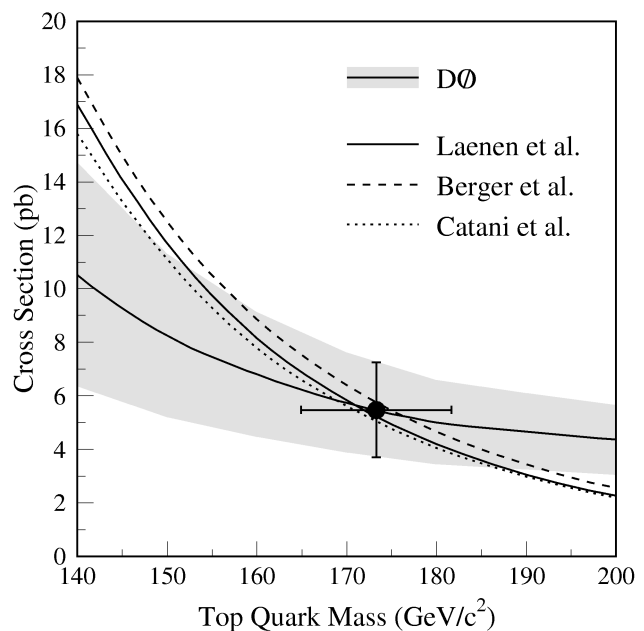
FIG. 3. Measured t\bar{t} production cross section as a function of m_t (shaded band). The point with error bars is the cross section for the measured top quark mass at D0. Three different theoretical estimates are also shown.
