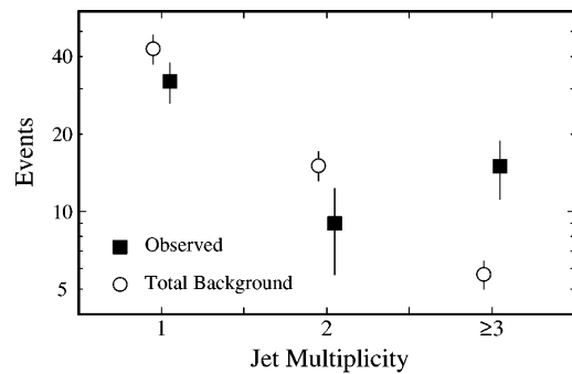
FIG. 2. Jet multiplicity spectrum of \ell + \text{jets}/\mu events before imposing event shape ( \mathcal{A}, H_T ) criteria, compared to background estimates.
