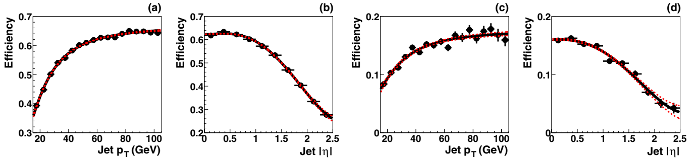
FIG. 8 (color online). Inclusive b tagging efficiency vs (a) jet p_T and (b) jet |\eta| and inclusive c tagging efficiency vs (c) jet p_T and (d) jet |\eta| . The resulting fit is shown as a solid line, and the \pm 1\sigma statistical uncertainty is shown as dotted lines.
