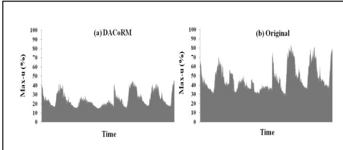
Figure 3. Evolution of max-u at 15 minute intervals using (a) DACoRM, and (b) Original scheme, for the GEANT network
