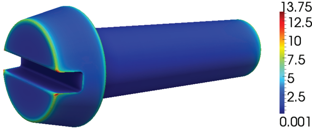
Fig. 5. Charge density (in \text{nC}/\text{m}^2 ) on the surface of a 13-mm-long bolt held at the potential u = 1 \text{ V} .
