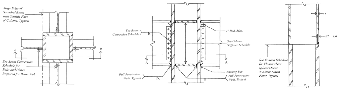
A. Plan Section Typical Connection B. Typical Moment Connection C. Typical Splice
