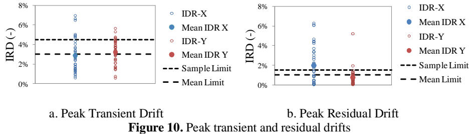
Figure 10. Peak transient and residual drifts
