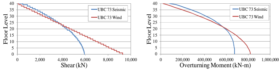
Figure 3. Cumulative wind and seismic base shears and overturning moments per UBC 73
