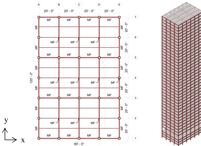
Figure 2. Prototype 40-story office building
