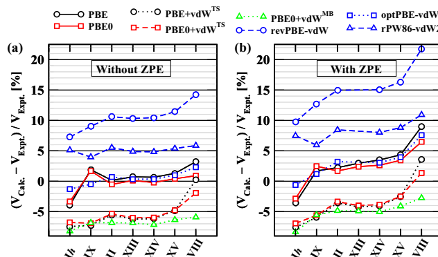
FIG. 3. Percentage differences in the calculated equilibrium volumes ( V_{\text{Calc.}} ) compared to experiment ( V_{\text{Expt.}} ) (a) without and (b) with zero point energies (ZPE) in V_{\text{Calc.}} . The zero value on the Y axis designates the experimental reference values. Here positive errors indicate larger computed volumes and negative errors indicate smaller computed volumes compared to experiment.
