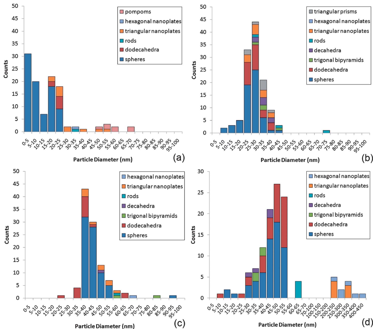
Fig. 6 Histogram plots of nanoparticle size (nm) and count for the various nanostructures observed after (a) 5 minutes, (b) 20 minutes and (c) 65 minutes of reaction from the self-initiated gold nanoparticle formation reaction of auric acid solution and cyclohexanone and (d) after 3 months storage.
