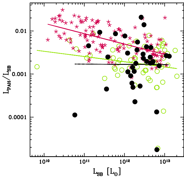
Figure 9. SFR_{\text{FIR}} versus SFR_{\text{PAH}} (top) and L_{\text{PAH}}/L_{\text{SB}} as a function of L_{\text{SB}} (bottom) for unobscured AGN-dominated objects (filled circles), AGN-dominated objects with an optical stellar component (open circles) and starburst-dominated objects (stars). The continuous lines mark the respective linear correlations and the dashed line (top panel) the 1:1 relation.
