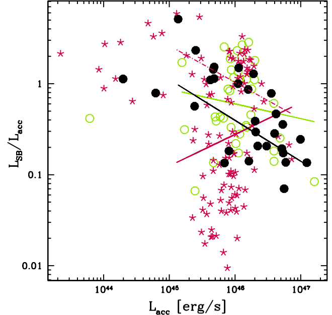
Figure 10. SFR_{\text{FIR}} versus L_{\text{acc}} and L_{\text{SB}}/L_{\text{acc}} as a function of L_{\text{acc}} for unobscured AGN-dominated objects, AGN-dominated objects with an optical stellar component and starburst-dominated objects. The symbol code is the same as in Fig. 9. The linear correlations shown here are computed for objects with L_{\text{acc}} > 10^{45} \text{ erg s}^{-1} alone. The dotted lines represent the correlation for starburst-dominated objects when discarding sources with N_{\text{H}} < 3 \times 10^{23} \text{ cm}^{-2} .
