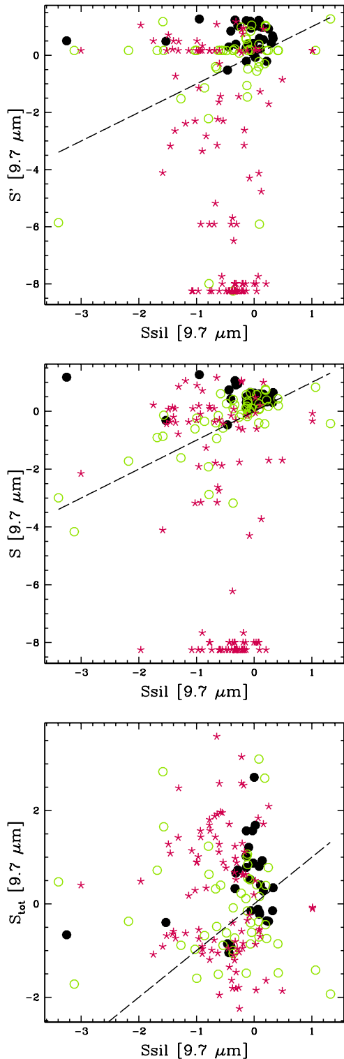
Figure 7. The strength of the silicate feature at 9.7\ \mu\text{m} measured from the best-fitting model versus that measured from the IRS spectra. In the top panel, S' was measured on the best-fitting torus models obtained by fitting photometry alone, while S (middle panel) was measured from the best-fitting torus model when fitting simultaneously photometric data and IRS spectra. In the bottom panel, S_{\text{tot}} is the measured strength of the silicate feature on the total model, i.e. the sum of the AGN and the starburst component. The filled black (open green) circles correspond to AGN-dominated objects without (with) a stellar component (SSPs), while the red stars correspond to starburst-dominated objects.
