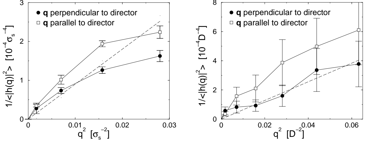
Figure 1: Inverse mean-squared Fourier components of the interface position h vs. wave vector \mathbf{q} squared for \mathbf{q} parallel and perpendicular to the director \mathbf{n}_0 . Left: Ellipsoids (similar to Ref. 6; data taken from Ref. 15). Right: Hard rods (similar to Ref. 9, different data set). The straight dashed lines indicate the prediction of Eq. (2) with the interfacial tension taken from Table 1, \gamma = 0.009k_B T/\sigma_s^2 (ellipsoids) and \gamma = 0.0064k_B T/D^2 (hard rods). Remarkably, it seems to fit the lower branch ( \mathbf{q} \perp \mathbf{n}_0 ) rather well in both systems.
