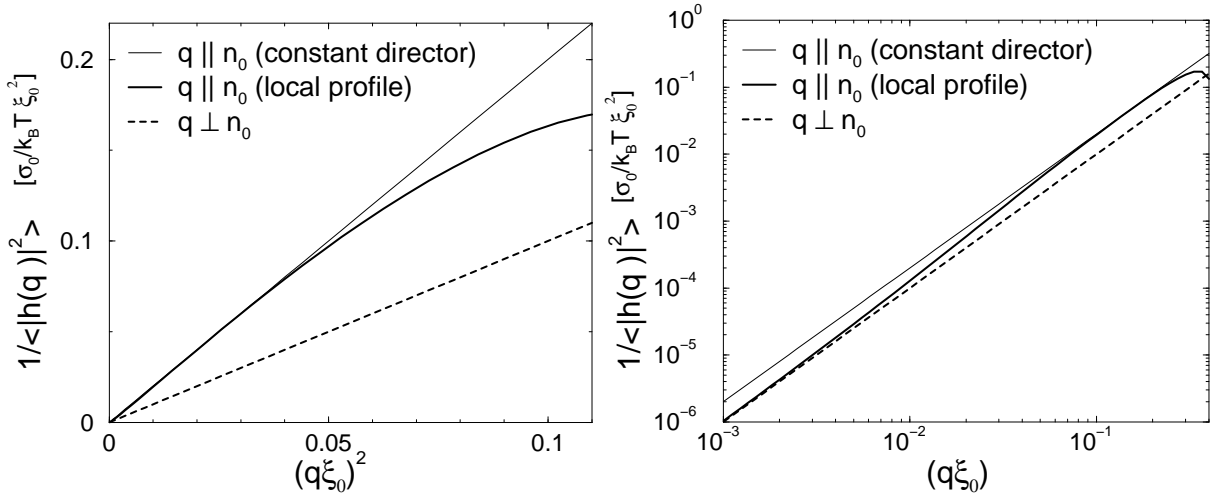
Figure 2: Capillary wave spectrum in the direction parallel and perpendicular to the director as predicted by the theory for \alpha = 1 . The thin solid line corresponds to the constant director approximation, Eqs. (12) and (13), the thick solid line to the local profile approximation. In the direction perpendicular to the director, both approximations give the same result, which also agrees with the prediction for simple fluid interfaces, Eq. (2). Left: Linear plot vs. q^2 . Right: Double logarithmic plot showing the crossover between isotropic and anisotropic behavior.
