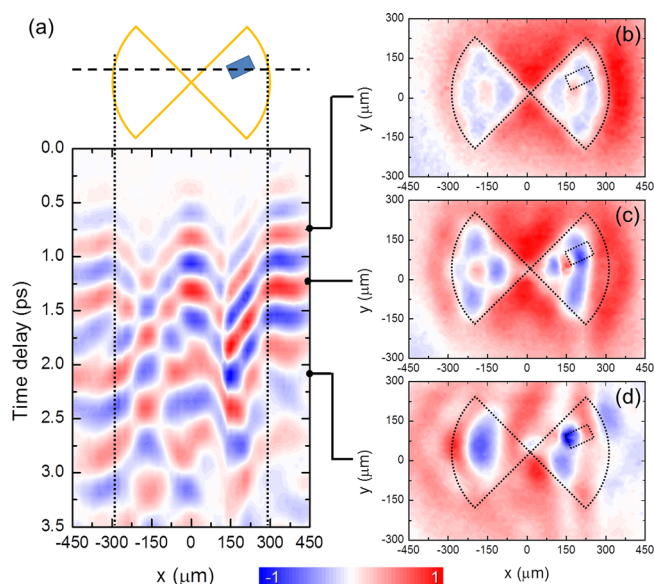
FIG. 2. (a) Measured temporal evolution of the detected signal along the horizontal line outlined in the diagram at z \sim 25 \mu\text{m} . (b)-(d) THz near-field images for selected time delays indicated on the xt -map. The bow-tie and the STO particle are outlined with dotted lines.
