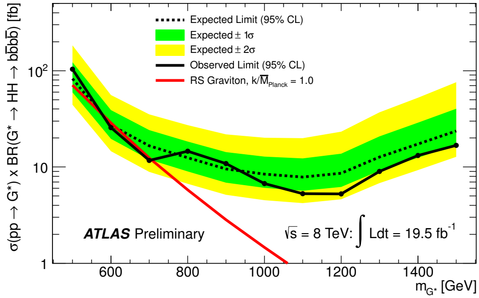
Figure 4.32.: The expected and observed upper limits on the RS graviton cross section \times branching ratio in the HH channel.
