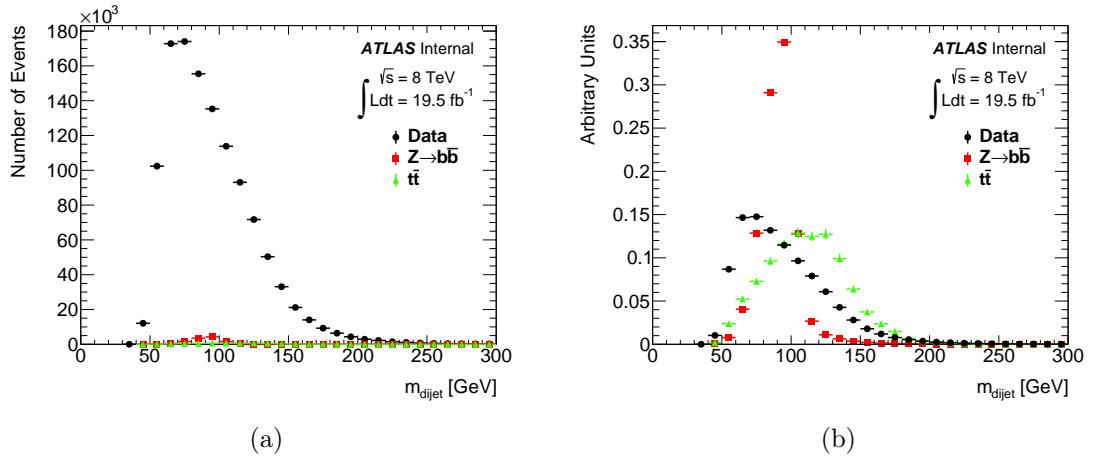
Figure 3.4.: The dijet mass distribution of events passing the preselection. (a) The MC is normalised to the predicted number of events (b) The MC and data are normalised to equal area.
