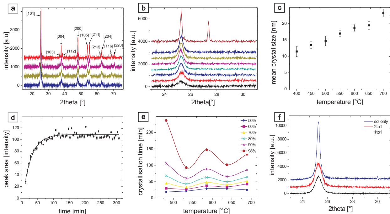
Figure 2: Crystallisation of TiO 2 anatase crystals in block-copolymer derived confinement (a) Wide angle x-ray diffraction scans of mesoporous films annealed at 400 °C, 500 °C, 600 °C, and 700 °C (bottom to top). (b) Anatase (101) crystal footprint as a function of crystallisation temperature after annealing for 400 min. From bottom to top: 400 °C to 700 °C in 50 °C increments (structurally intact), and 740 °C (collapsed structure). (c) Debye-Scherrer mean crystallite sizes after annealing for 400 min as a function of temperature. (d) Evolution of crystallinity by monitoring the peak area as a function of time at 530 °C. (e) Evolution of overall crystallinity with time as a function of temperature. (f) Dependence of anatase (101) peak on mass ratio of TiO 2 to block copolymer. From bottom to top; black: 1 to 1 mass ratio (mean crystallite size: 9.5 nm); red: 2 to 1 mass ratio (14.7 nm); blue: sol only (23.6 nm).
