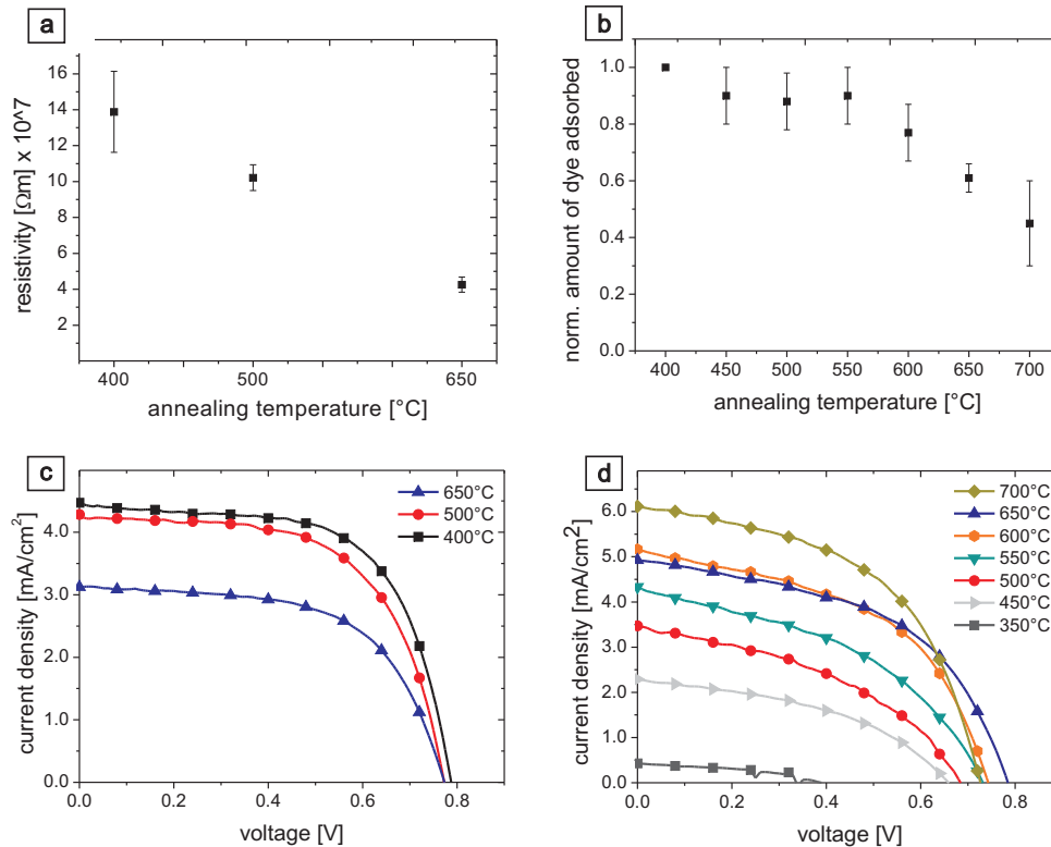
Figure 4: Effects of crystallinity on device performance. (a) Resistivity determined by impedance spectroscopy of 900 nm thick films annealed at 400 ^{\circ}\text{C} , 500 ^{\circ}\text{C} , and 650 ^{\circ}\text{C} . (b) Relative amount of dye adsorbed per unit area. The dye adsorption of the mesoporous film annealed at 400 ^{\circ}\text{C} was used as the baseline. (c) Current-voltage characteristics for liquid electrolyte DSC devices annealed at 400 ^{\circ}\text{C} , 500 ^{\circ}\text{C} , and 650 ^{\circ}\text{C} . (d) solid-state DSC performance of samples annealed at 350 ^{\circ}\text{C} to 700 ^{\circ}\text{C} . Higher temperatures led to a continuous increase in efficiency from 0.8% (450 ^{\circ}\text{C} ) to 2.5% (700 ^{\circ}\text{C} ) for 400 nm thick films sensitised with D102. Liquid and solid-state devices were characterised under standardised AM 1.5 illumination of 100 \text{W}/\text{cm}^2 . See the supporting information for a summary of all photovoltaic device performance parameters.
