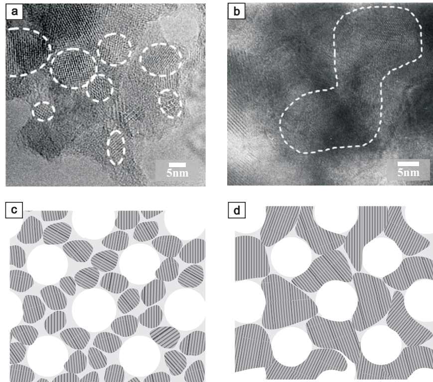
Figure 3: Crystallite assembly within the mesoporous network. High resolution transmission electron microscopy (HRTEM) images of samples annealed at (a) 400 °C and (b) 650 °C. White dotted lines are superimposed on the images to visualize individual crystallites. (a) Sample annealed at 400 °C: small, randomly oriented crystals significantly smaller than the lengthscale of the porous matrix are observed. (b) Sample annealed at 650 °C: crystal size exceeds the length scale of the confinement. Anisotropic growth within the network is likely. (c-d) Schematic illustrating crystallite size and orientation in copolymer derived networks at (c) 400 °C and (d) 650 °C.
