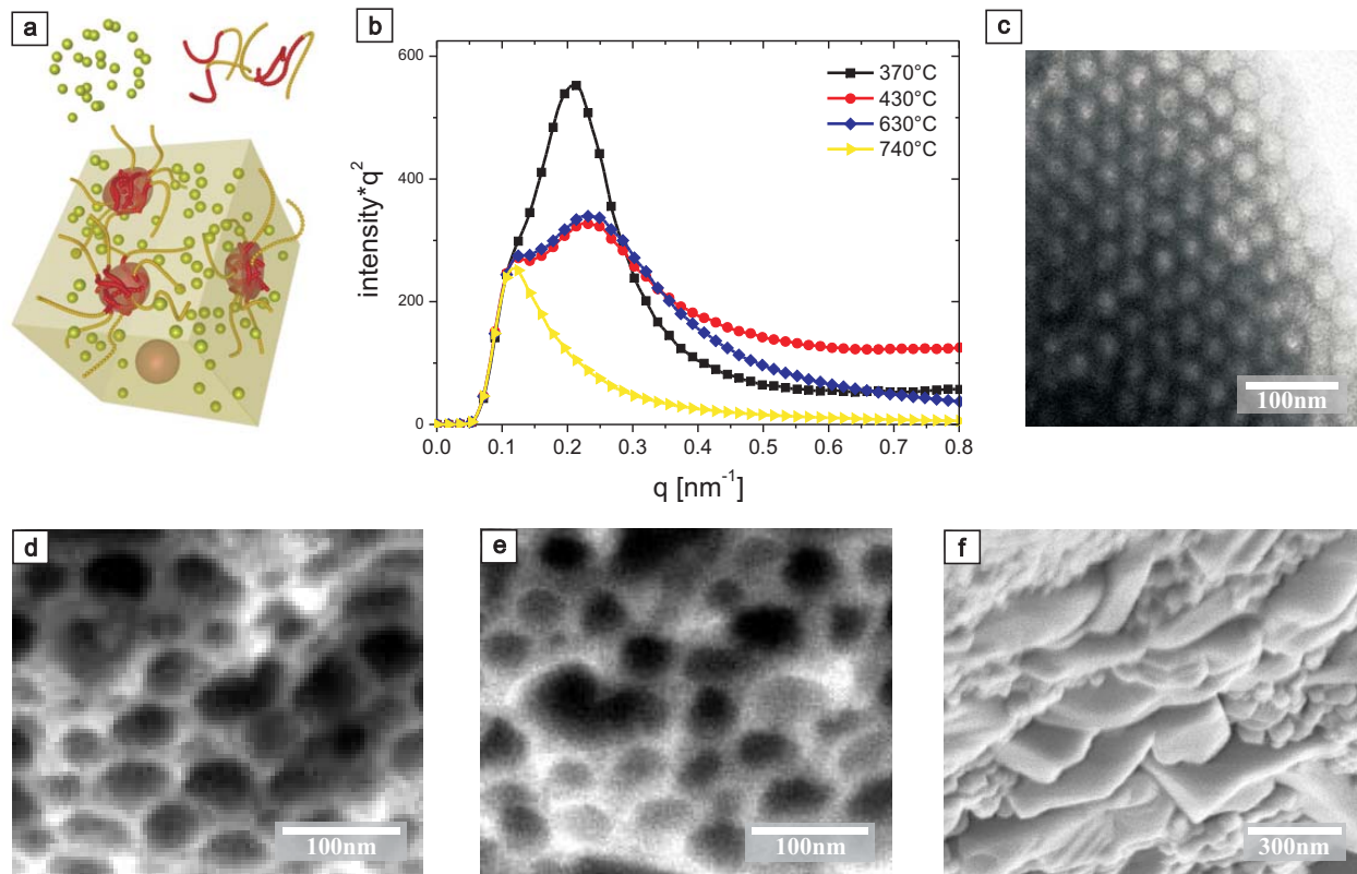
Figure 1: Film deposition and structural stability. (a) Hydrolytic TiO 2 sol when mixed with a PI- b -PEO solution is structure-directed by copolymer self-assembly, giving rise to nanostructured TiO 2 after high-temperature annealing. (b) Small-angle x-ray scattering (SAXS) spectra for copolymer-derived TiO 2 annealed at 370 °C (black squares), 430 °C (red circles), 630 °C (blue diamonds) and 740 °C (yellow triangles). The spectra are scaled in intensity to overlap in the 0 – 0.1 nm -1 q -range. (c) TEM image of the ordered f.c.c. micellar hybrid film produced by spin-coating the redissolved material. Cross-sectional SEM images of the nanostructured TiO 2 films calcined in air at temperatures of (d) 430 °C and (e) 690 °C for 400 min. (f) Cross-sectional SEM image of a film annealed at 740 °C which resulted in the transformation from anatase to rutile and a subsequent loss of the mesopores.
