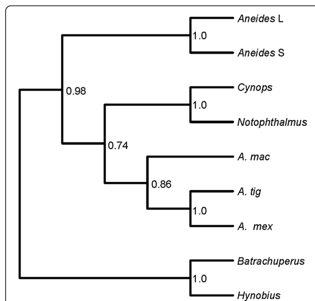
Figure 2 Phylogenetic tree for the Prod 1 sequences in Figure 1. Trees were computed by maximum likelihood and Bayesian inference, with equivalent results. Maximum likelihood trees were built using PhyML [21] and jModeltest [22] for model selection; support for clades was evaluated with 1,000 bootstrap pseudoreplicates. Bayesian analyses were carried out with MrBayes v.3.1.2 [23], for a total of 50,000 generations, sampling every 50 generations. Substitution models were estimated during the analysis by model-jumping with a proportion of invariable sites.
