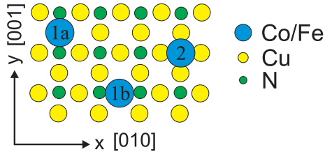
FIG. 1: Topview of the three adsorption sites populated by Fe and Co adatoms on \text{Cu}_2\text{N}/\text{Cu}(100)\text{-}c(2 \times 2) . 1a and 1b denote atop Cu sites with two orthogonal in-plane orientations of N-neighbors. 2 denotes the atop N site having fourfold in-plane symmetry.
