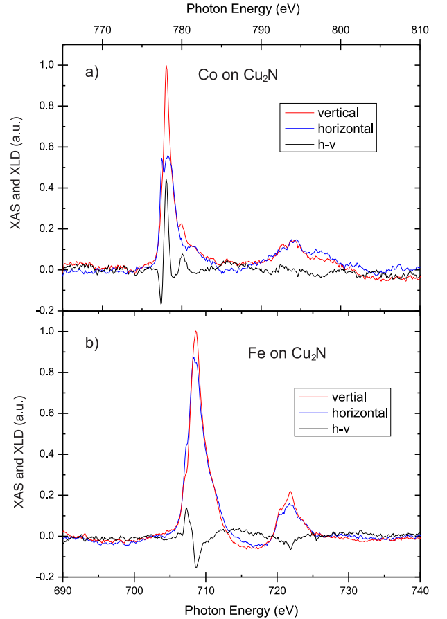
FIG. 6: XAS spectra recorded with linear polarization and their dichroism for Co (a) and Fe (b) on \text{Cu}_2\text{N} both measured at \theta = 70^\circ and B = 0.005 T . From the shown spectra the background as well as a step function for the non resonant absorption have been subtracted.
