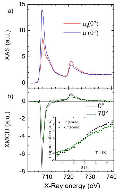
FIG. 4: a) Background corrected XAS for 0.02 ML Fe on \text{Cu}_2\text{N}/\text{Cu}(100)\text{-c}(2 \times 2) ( \theta = 0^\circ , B = 5 T, T = 8 K). b) Corresponding angular dependent XMCD. The insert displays magnetization curves obtained as in Fig. 1 b).
