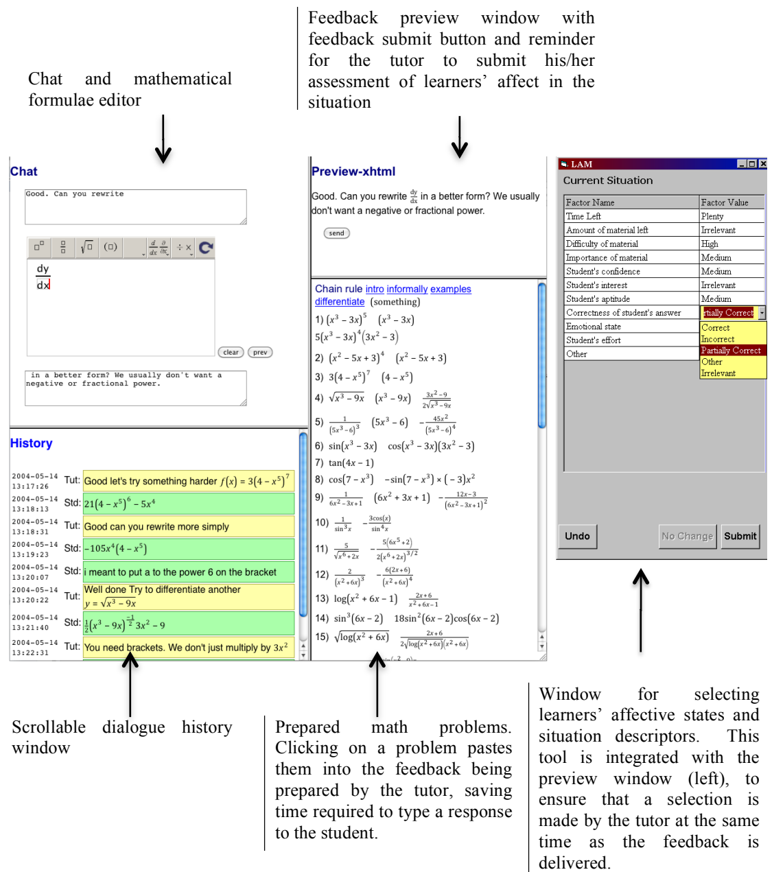
Figure 2: Dialogue and data collection interface used in Porayska-Pomsta, Mavrikis and Pain (2008) studies.
