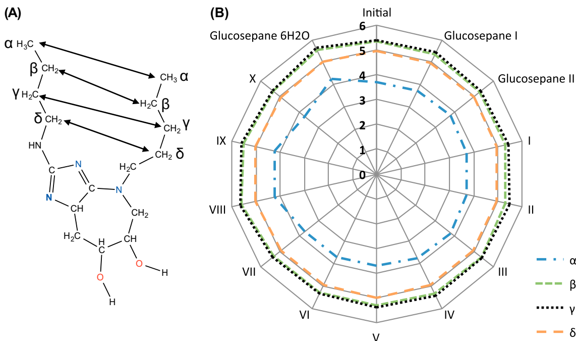
Figure 2. A distance comparison between interatomic carbon atoms along the aliphatic chain of lysine and arginine. (A) The structure of glucosepane (with methyl capping in place of the \alpha -carbon atoms). Carbon atoms along the length of each aliphatic chain are denoted \alpha , \beta , \gamma and \delta . The \epsilon carbon on lysine lacks comparison given the shorter length of arginine. (B) A measure of interatomic carbon distances per complex, per glucosepane structure and for the initial MD simulation structure. Note: The graph radius denotes distance in Å.
