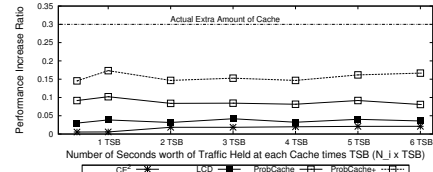
(b) Scenario 2.2: Larger Cache at the Edge ( c \rightarrow E )
