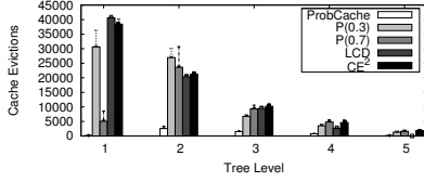
Fig. 3. Scenario 1: Average Number of Cache Evictions per Tree Level
