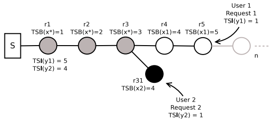
Fig. 1. Design Topology
