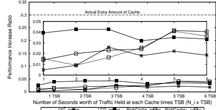
(a) Scenario 2.1: Larger Cache at the Core ( C \rightarrow e )
