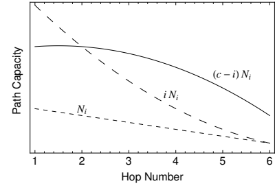
Fig. 4. Path Capacity calculation that takes place at each router along a 6-hop Path: the N_i curve is for homogeneous caches, hence the capacity is given by c \rightarrow e : \sum_{i=1}^{c-(x-1)} N_i ; the iN_i curve is for larger core caches, hence C \rightarrow e : \sum_{i=1}^{c-(x-1)} iN_i ; the (c-i)N_i curve is for larger caches towards the edge, hence c \rightarrow E : \sum_{i=1}^{c-(x-1)} (c-i)N_i .
