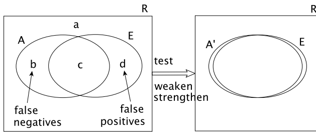
Figure 1: Assertion improvement process: the intersection between states where \langle \mathit{assert} \rangle is true ( A ) and expected states ( E ), restricted to the subset of reachable states ( R ), is increased.
